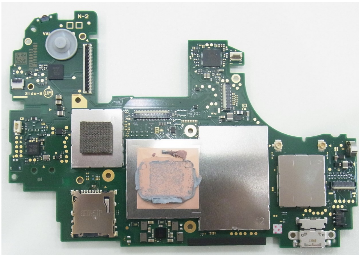
Wireless module PCB (Front, Shielded):
