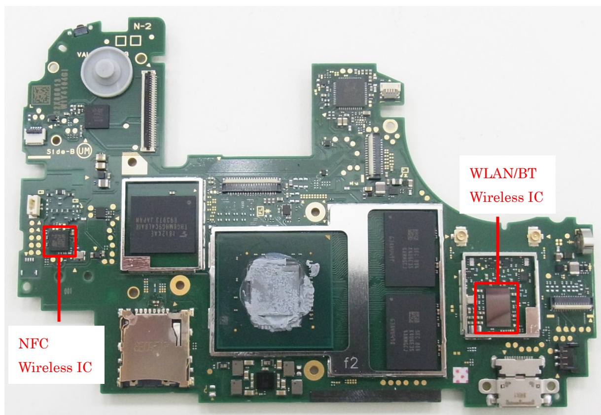
Wireless module PCB (Front, Shield removed):
