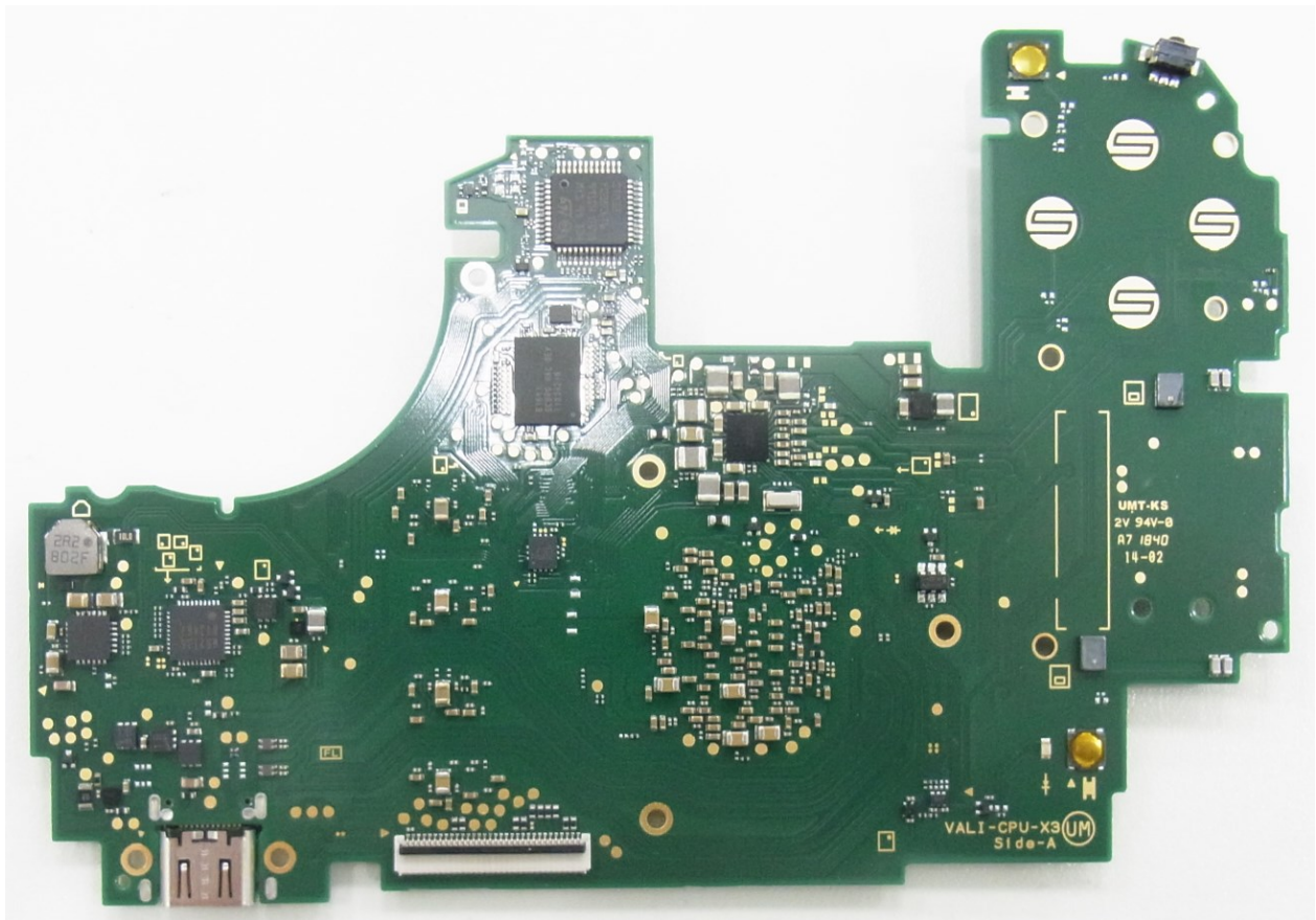
Wireless module PCB (Back):
