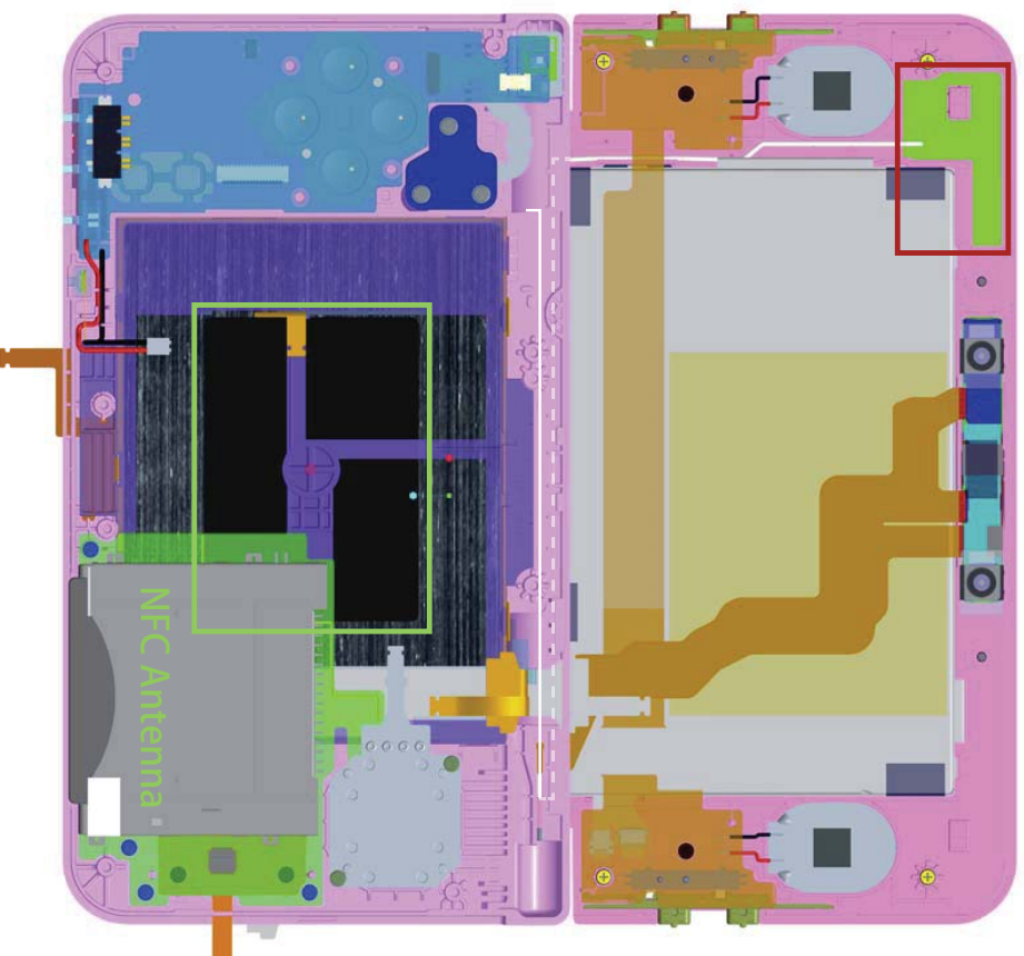
Wi-Fi Antenna
