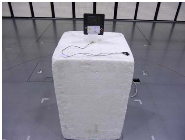
Rear (9kHz-30MHz)
