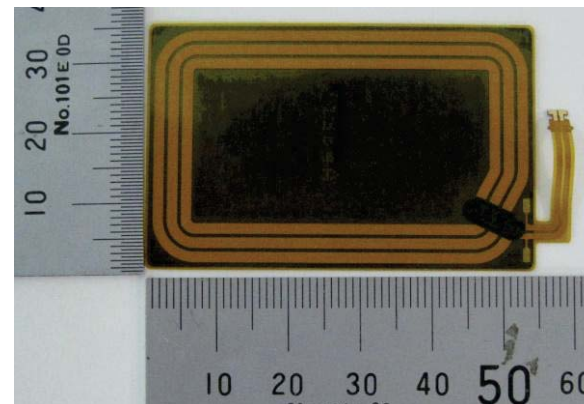
ANT/NFC-RED
