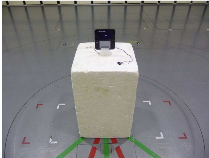
Rear (9kHz-30MHz)
