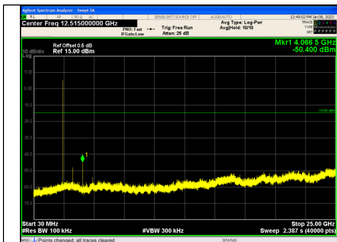
Spurious Emissions LE Coded (S=8) Channel 19
