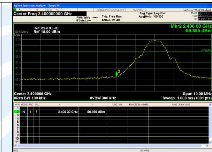
Out Of Band Emission LE Coded (S=2)_Channel 0
