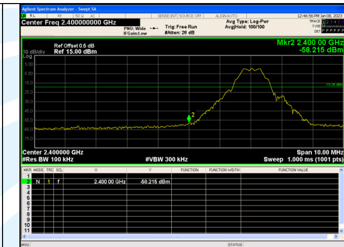
Out Of Band Emission LE Coded (S=8)_Channel 0
