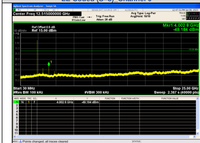
Spurious Emission LE Coded (S=8)_Channel 0
