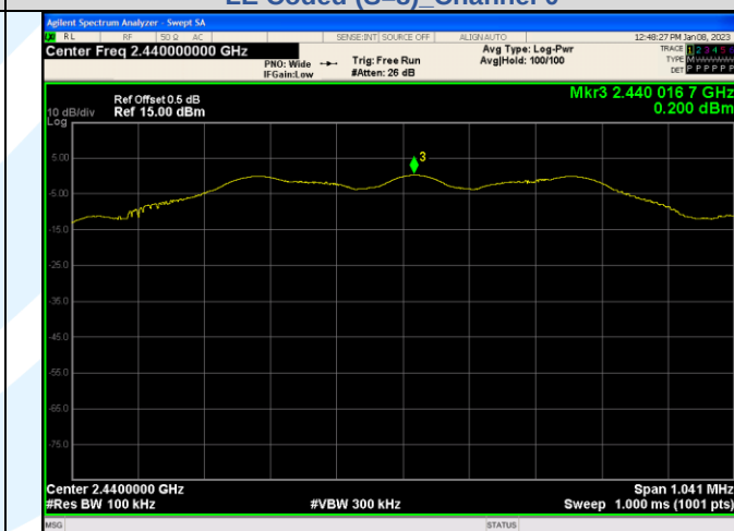
In-Band Reference Level LE Coded (S=8)_Channel 19
