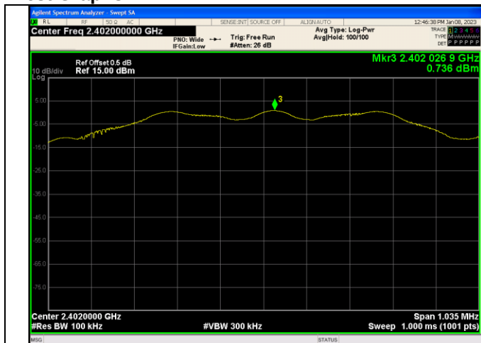
In-Band Reference Level LE Coded (S=8)_Channel 0
