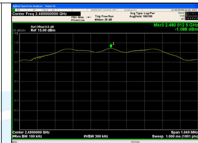
In-Band Reference Level LE Coded (S=8) Channel 39
