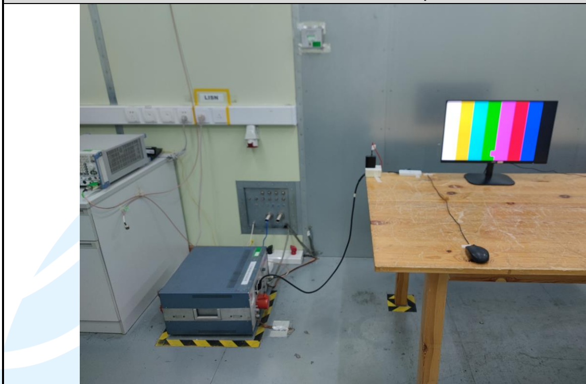
Conducted Emission Test Setup-3
