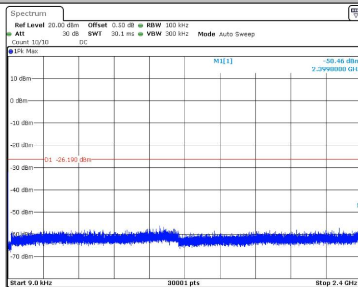
11N20SISO_ANT0_2412_0.009~2400
