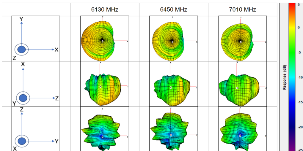
Radiation pattern _ ANT1 _ With 50 ohm
