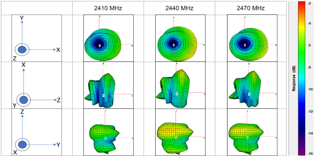
Radiation pattern _ BT _ With 50 ohm
