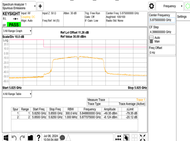
802.11n_40MHz_Chain0_5875MHz
