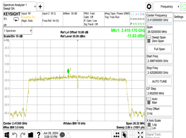
802.11ax_20MHz_Chain1_2412MHz_RU106_53
