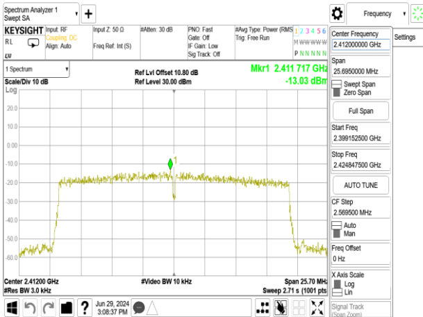
802.11ax_20MHz_Chain0_2412MHz_RU106_53
