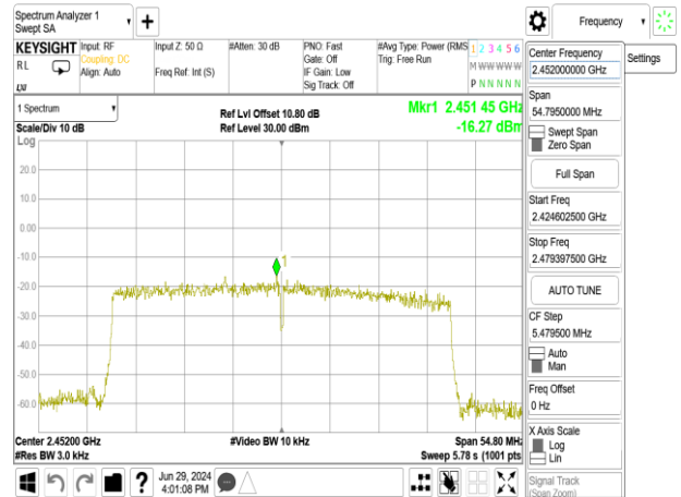
802.11ax_40MHz_Chain0_2452MHz_RU242_62
