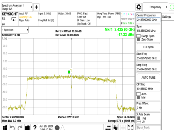
802.11ax_40MHz_Chain0_2437MHz
