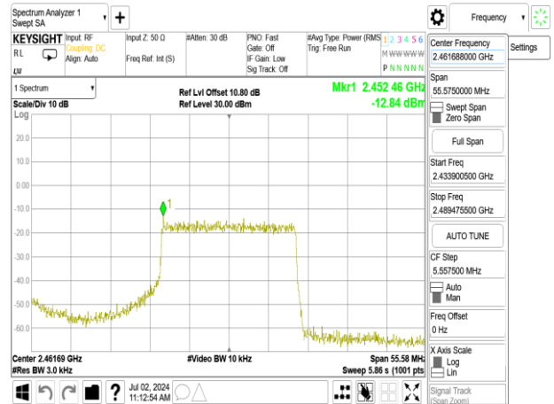
802.11ax_40MHz_Chain1_2452MHz_RU242_62
