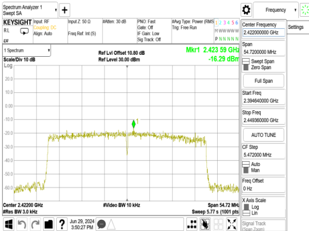
802.11ax_40MHz_Chain0_2422MHz_RU242_61
