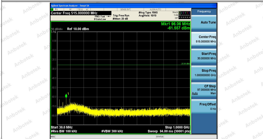
BLE_1M_Ant1_2442_30~1000
