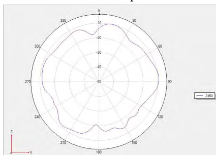
Phi =90 freq=2450MHz
