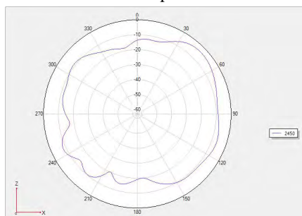
Phi =0 freq=2450MHz
