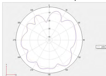
Theta =90 freq=2450MHz
