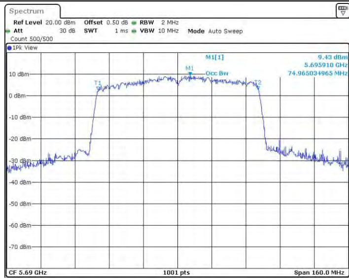
11AC80SISO_Ant2_5690
