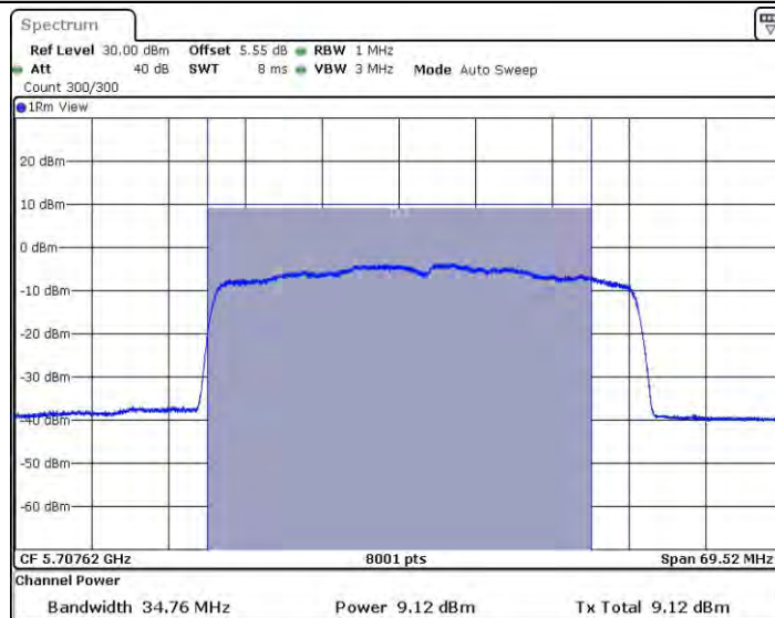
11AX40SISO_Ant1_5710_UNII-2C
