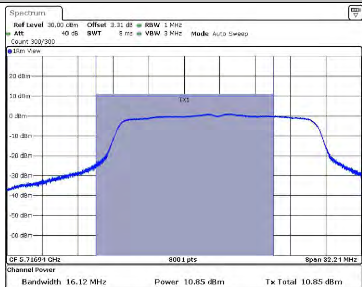
11AC20SISO_Ant2_5720_UNII-2C
