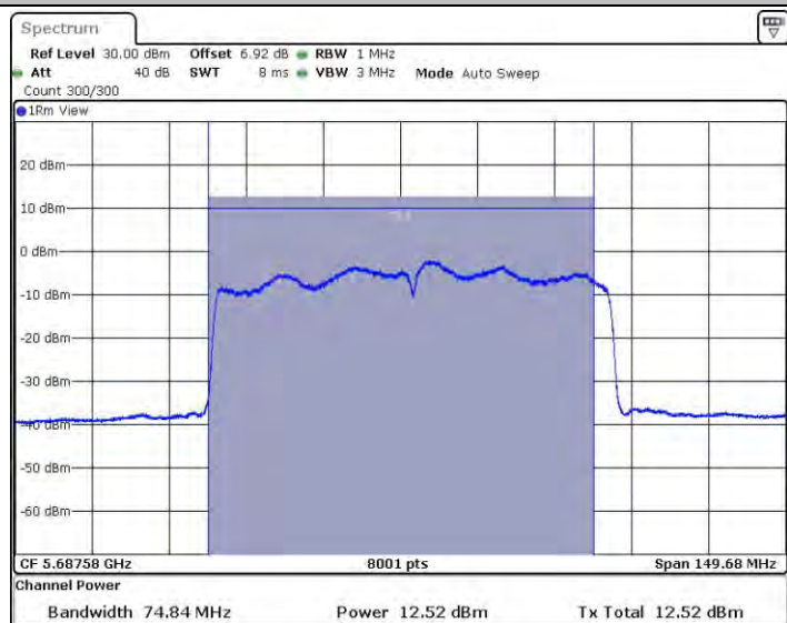
11AC80SISO_Ant2_5690_UNII-2C
