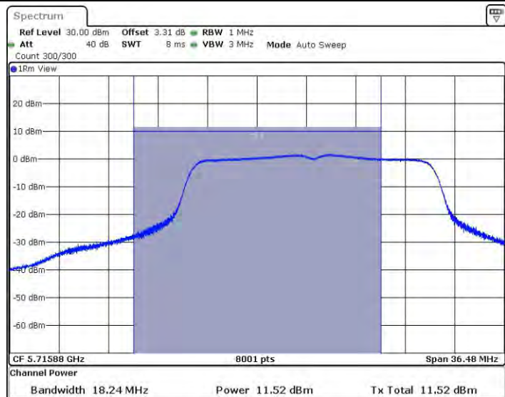
11AC20SISO_Ant1_5720_UNII-2C
