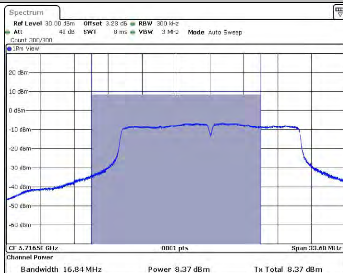
11AC20MIMO_Ant1_5720_UNII-2C
