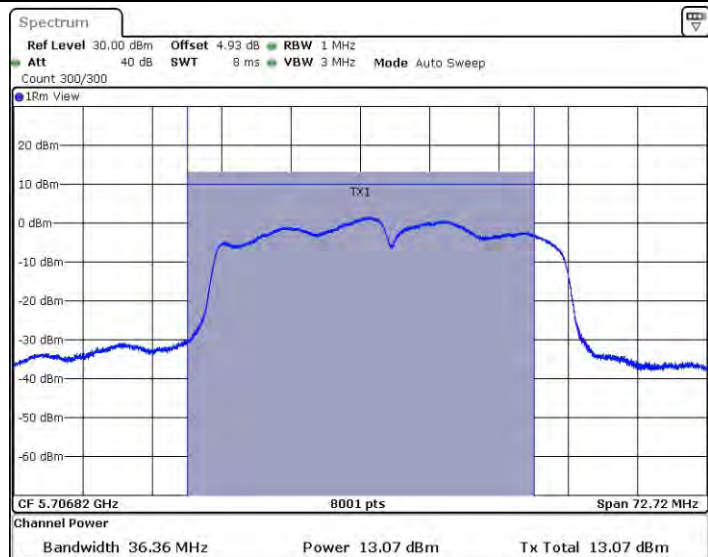
11AC40SISO_Ant1_5710_UNII-2C
