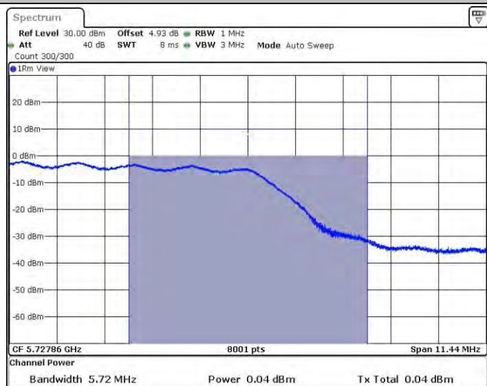
11AC40SISO_Ant1_5710_UNII-3
