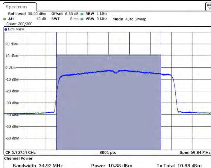
11AX40SISO_Ant2_5710_UNII-2C
