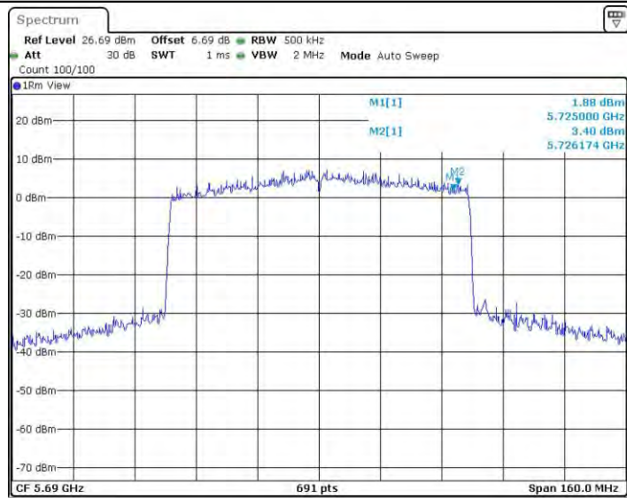
11AX80SISO_Ant2_5690_UNII-3
