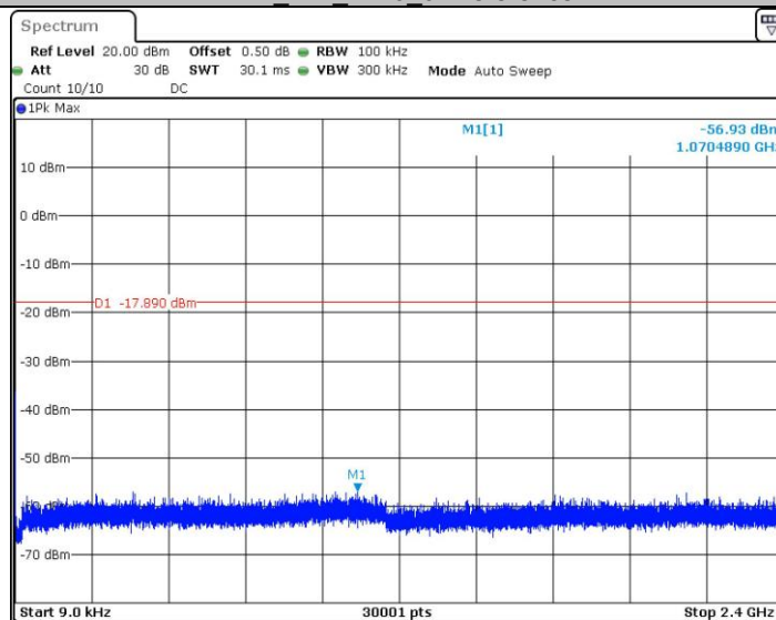
BLE_1M_2440_0.009~2400
