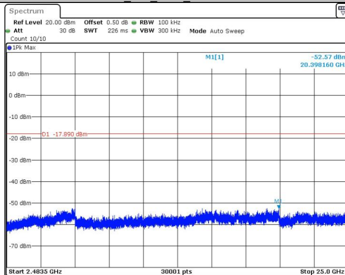
BLE_1M_2440_2483.5~25000
