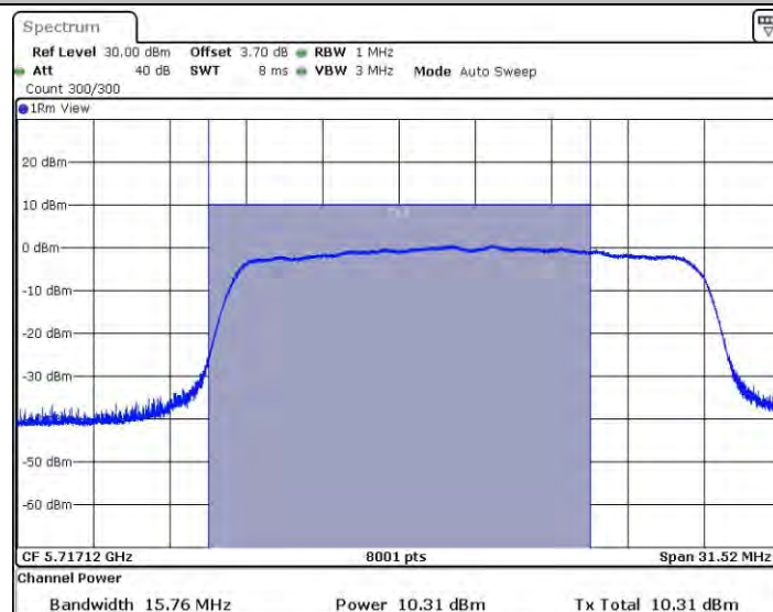
11AX20SISO_Ant2_5720_UNII-2C
