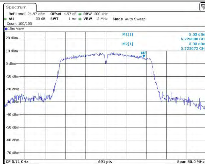
11AC40SISO_Ant1_5710_UNII-3
