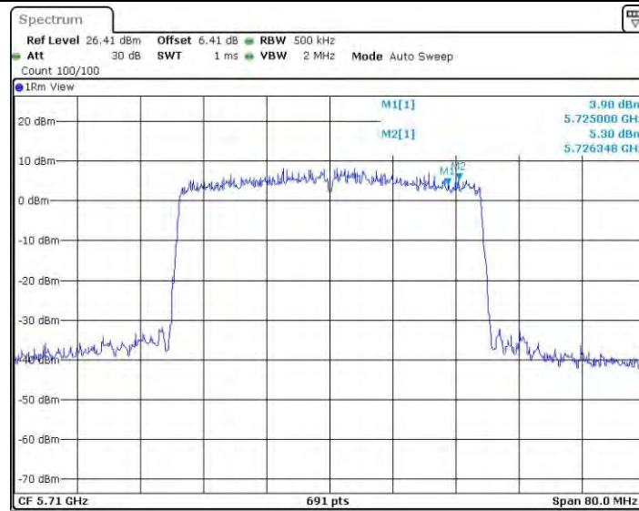
11AX40SISO_Ant1_5710_UNII-3
