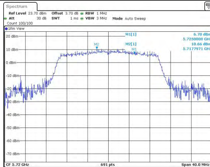
11AX20SISO_Ant1_5720_UNII-2C
