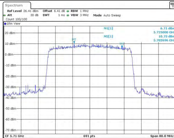
11AX40SISO_Ant1_5710_UNII-2C
