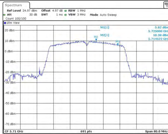
11AC40SISO_Ant1_5710_UNII-2C
