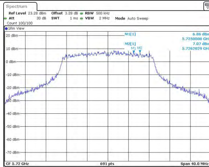
11AC20SISO_Ant2_5720_UNII-3
