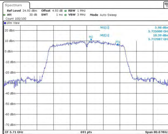
11AC40SISO_Ant2_5710_UNII-2C
