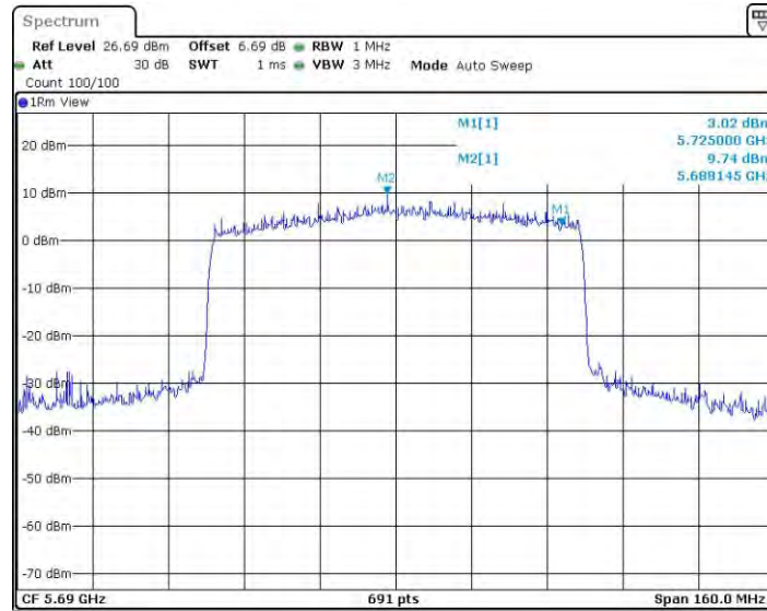
11AX80SISO_Ant2_5690_UNII-2C
