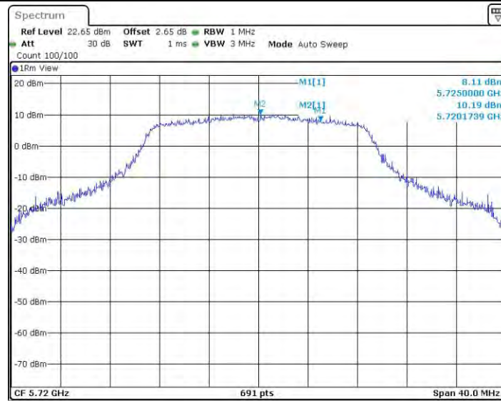
11AC20SISO_Ant1_5720_UNII-2C
