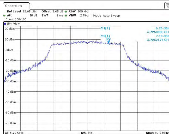
11AC20SISO_Ant1_5720_UNII-3
