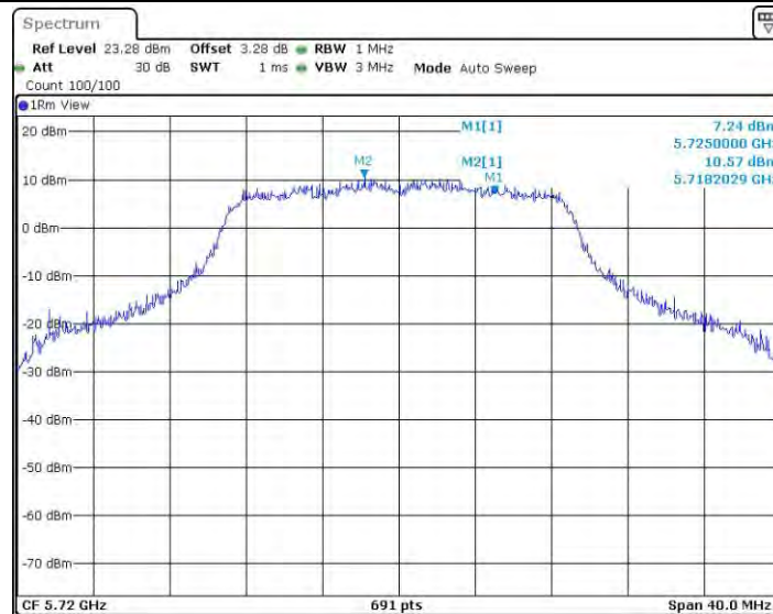
11AC20SISO_Ant2_5720_UNII-2C
