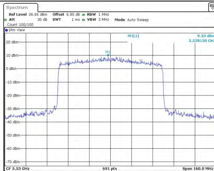
11AX80SISO_Ant2_5530
