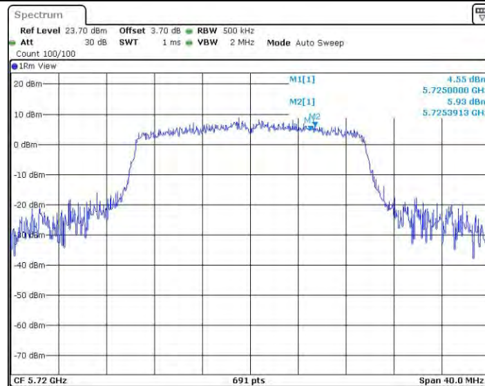
11AX20SISO_Ant2_5720_UNII-3
