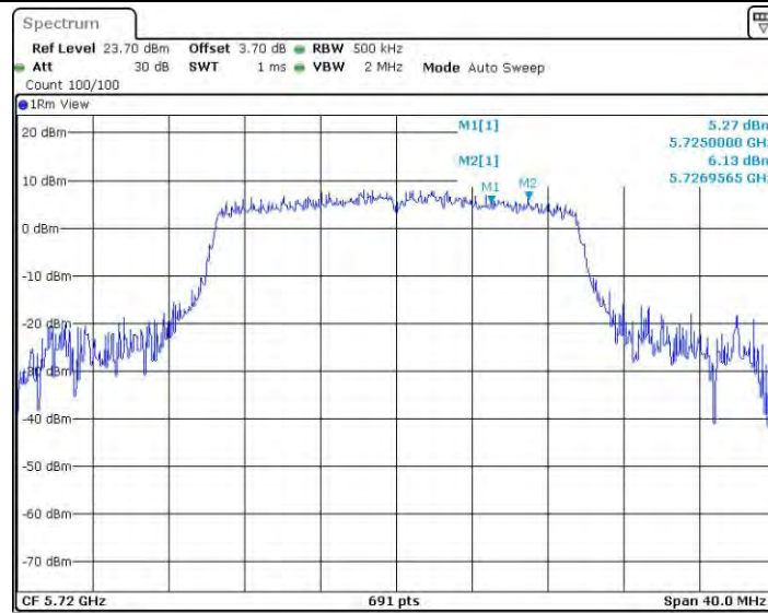
11AX20SISO_Ant1_5720_UNII-3
