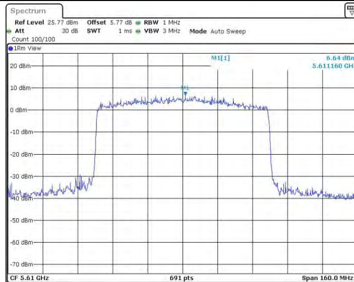
11AX80SISO_Ant2_5610
