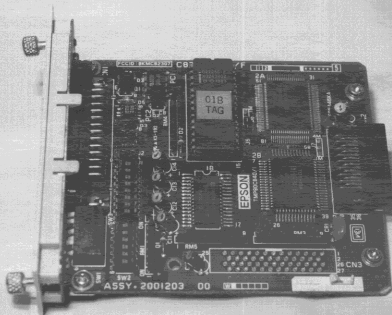
FCC ID BKMFBXYA-1 21) Optional Serial Interface card (SURFACE)
