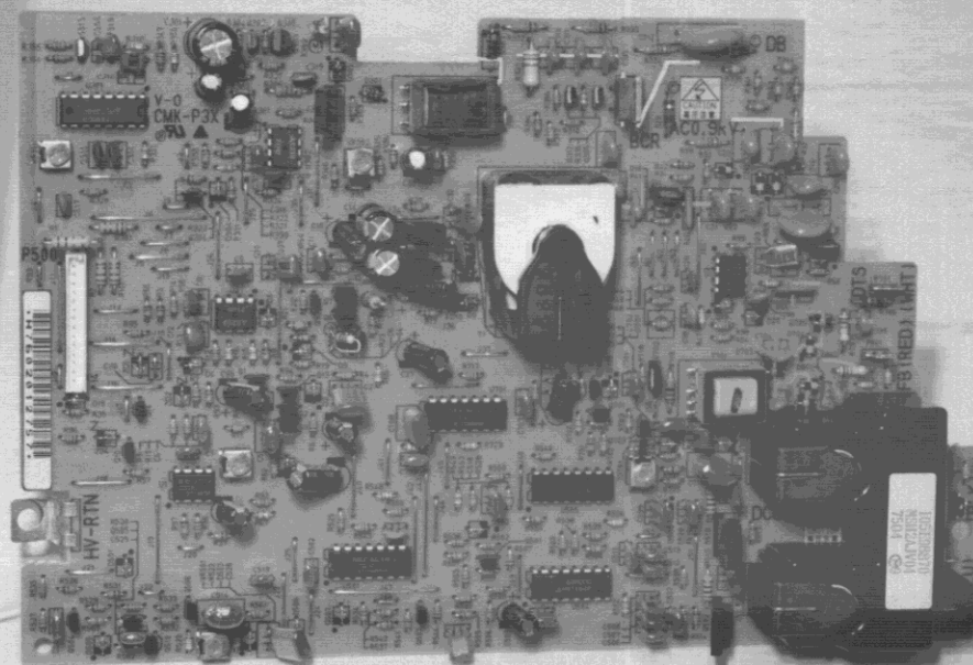
FCC ID BKMFBXYA-1 25) High Voltage Power Supply Board (SURFACE)
