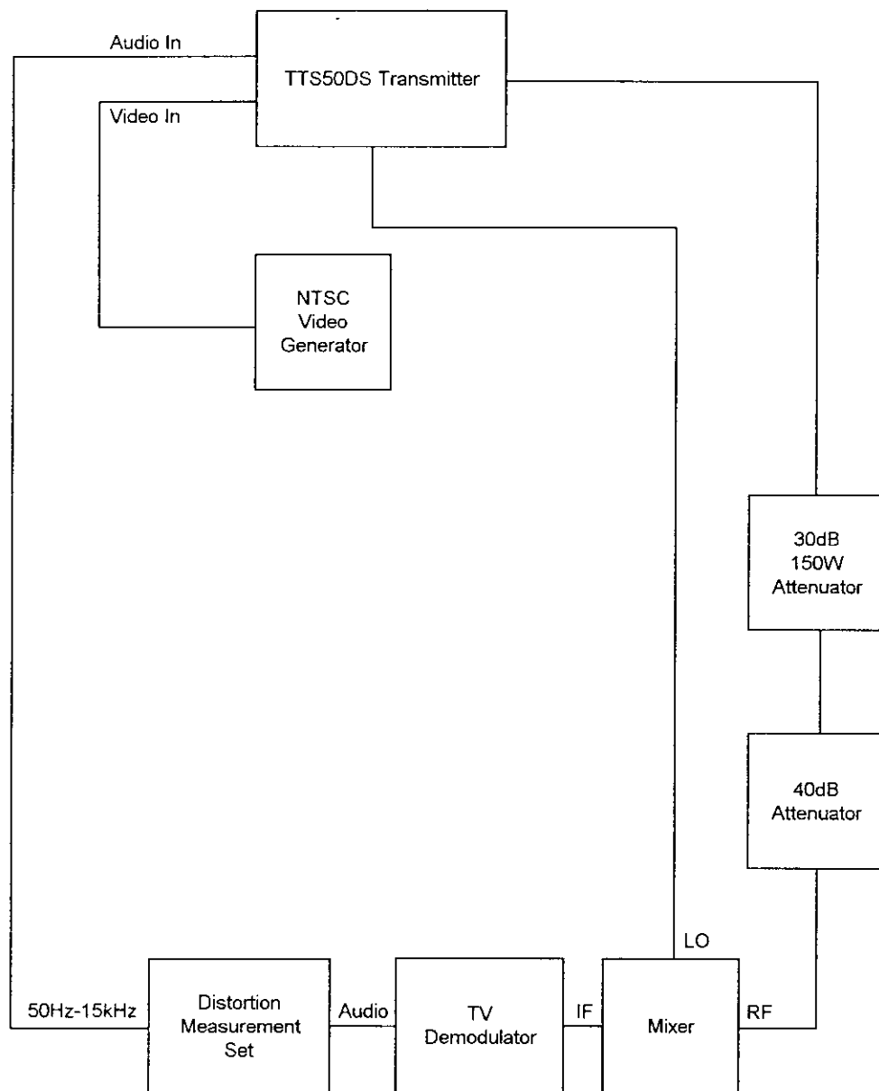
AURAL PRE-EMPHASIS TEST SETUP Figure 2-7A
