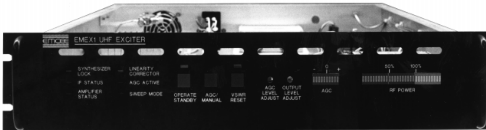
EMEX1 2 Watt UHF Exciter Front
