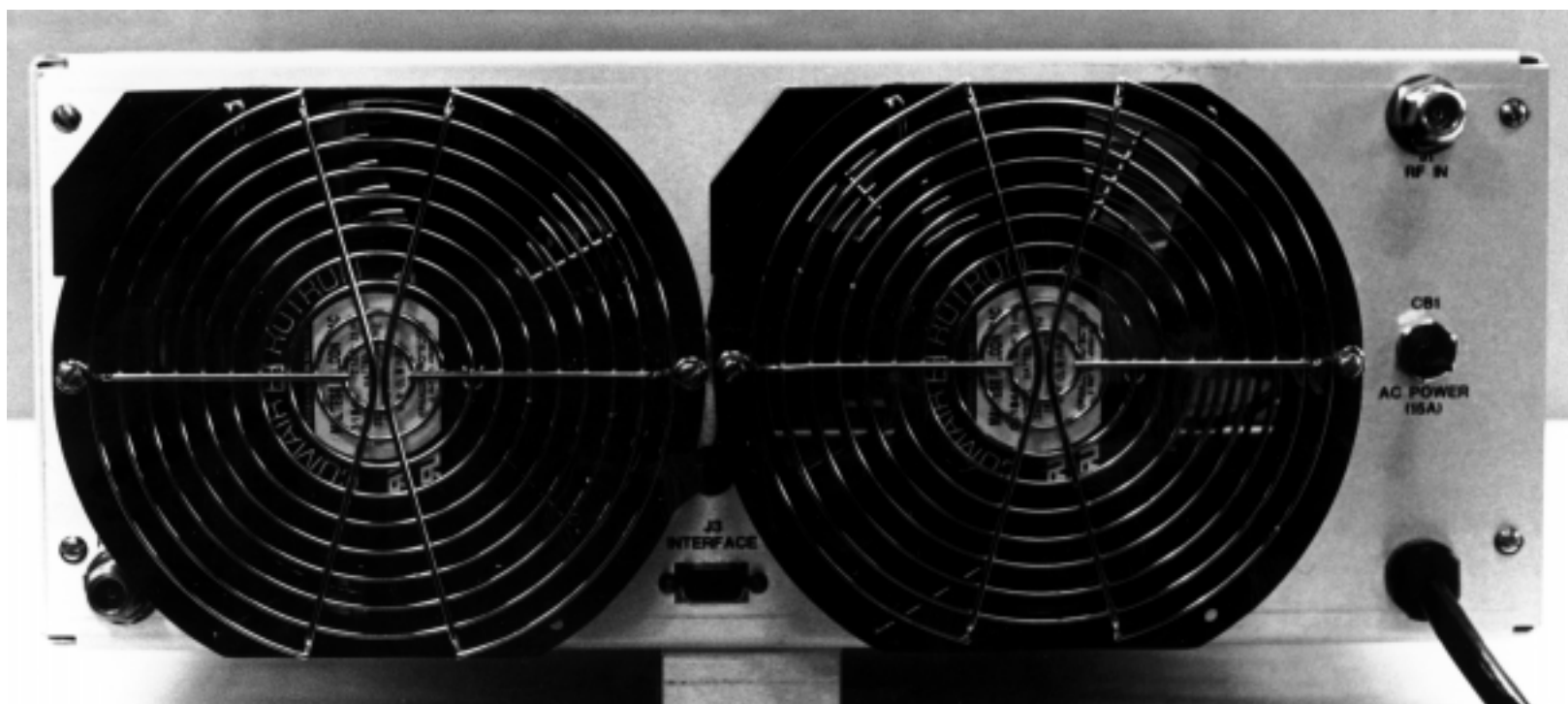
500W UHF Amplifier Drawer Rear
