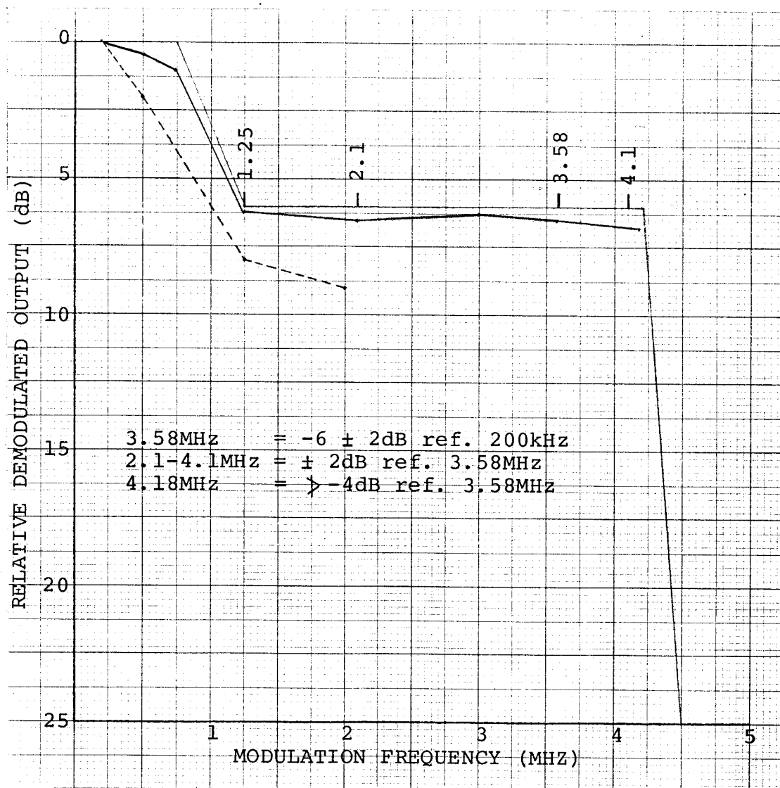
ATTENUATION CHARACTERISTICS CURVE
