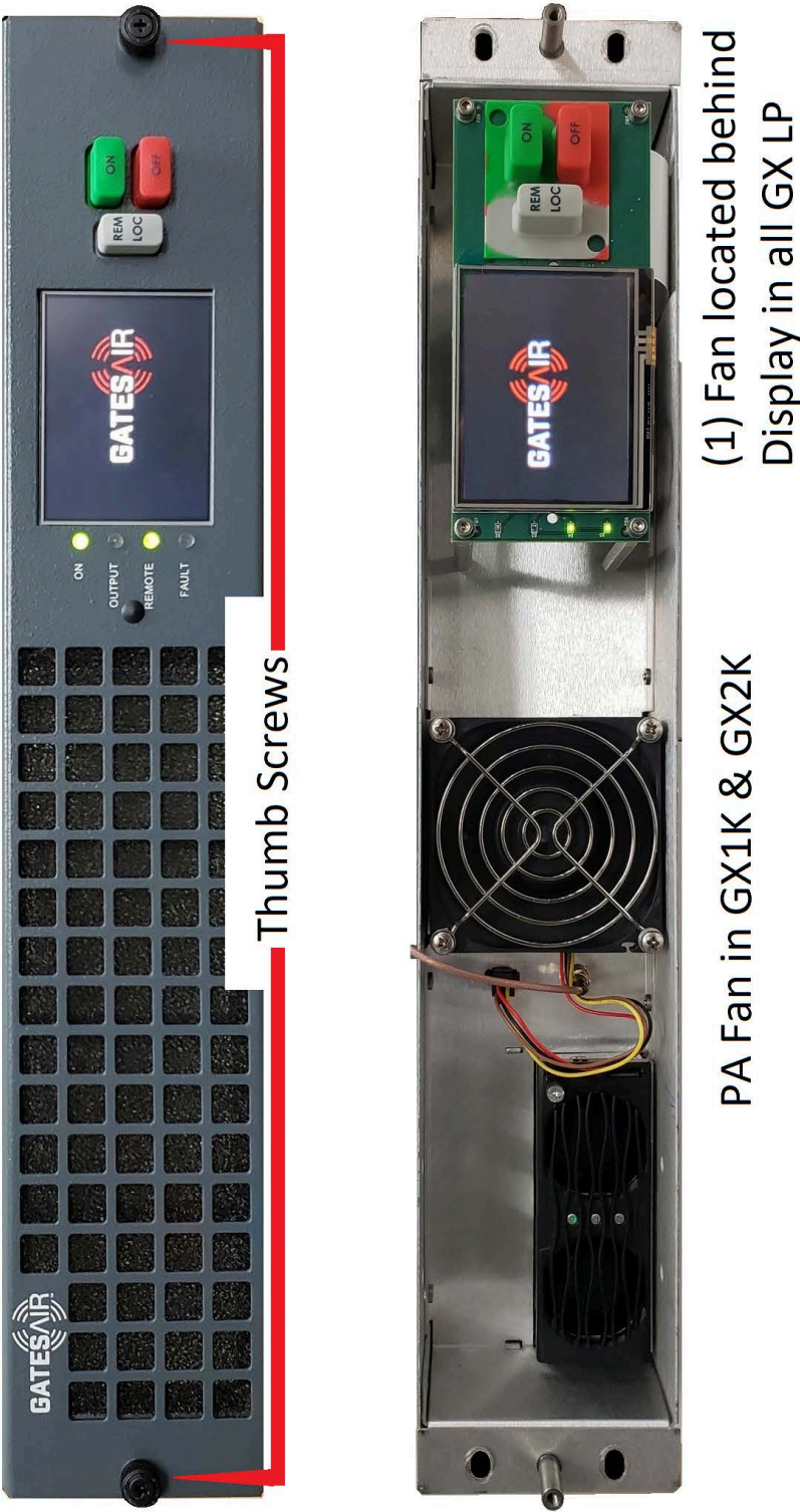
Figure 6-4 GX with Front Cover Removed
