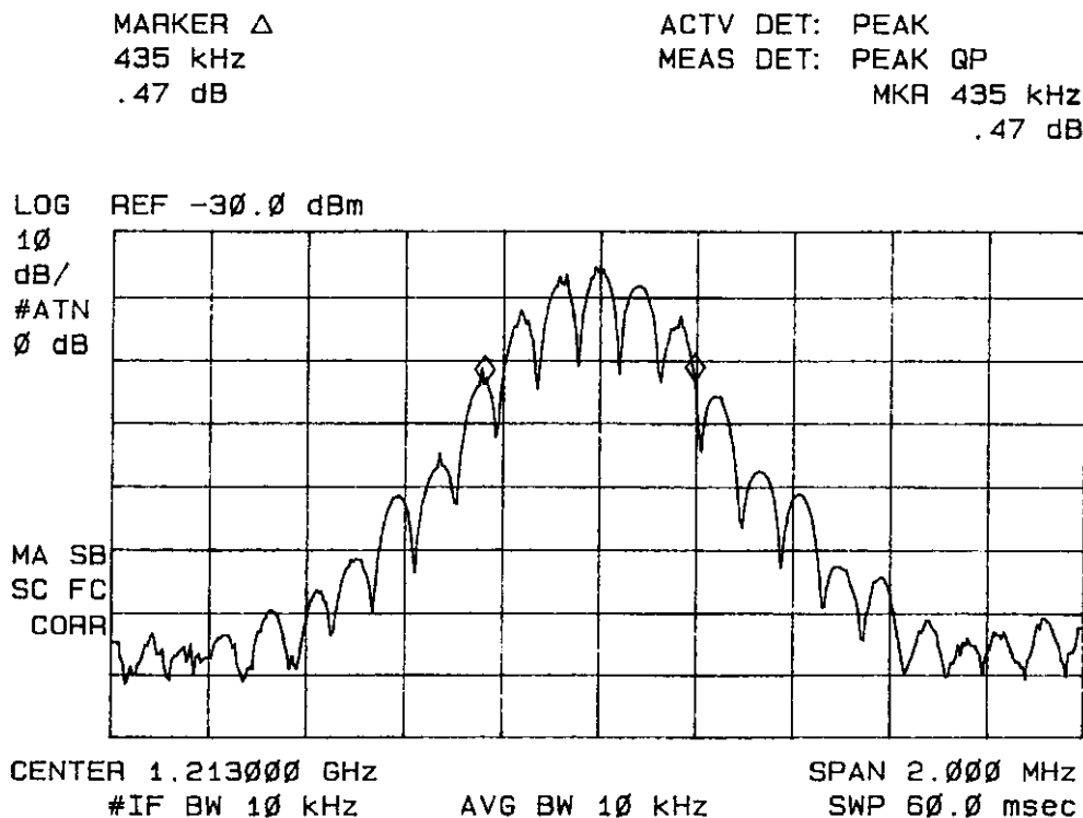
Figure 2 Occupied Bandwidth 1213 MHz
