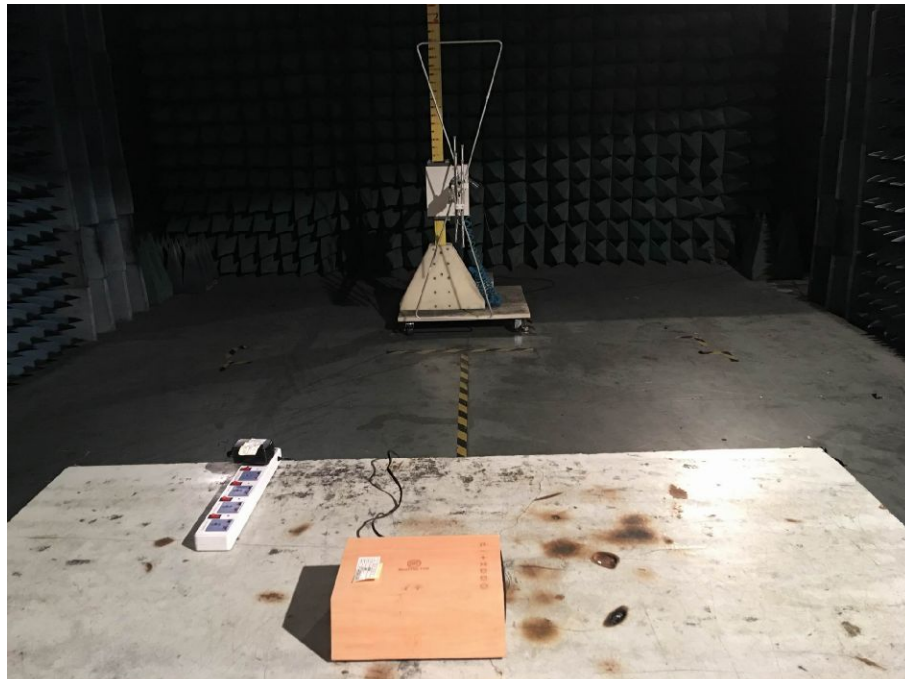
RE TEST SETUP PHOTO(30MHz-1000MHz)
