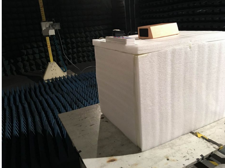
RE TEST SETUP PHOTO(ABOVE 1000MHz)
