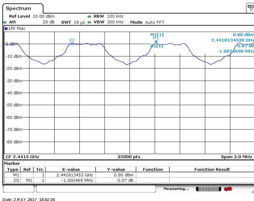
(Plot 4.6.1 A: Channel 39: 2441MHz @ GFSK)
