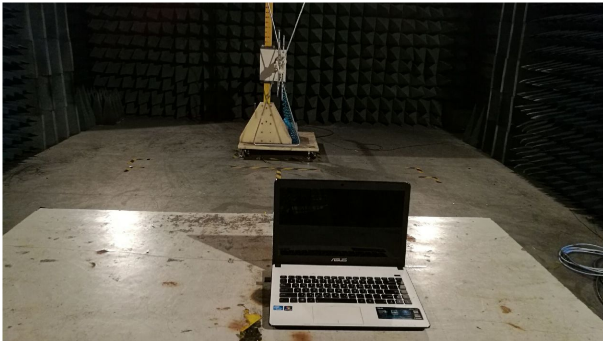
Above 1GHz
