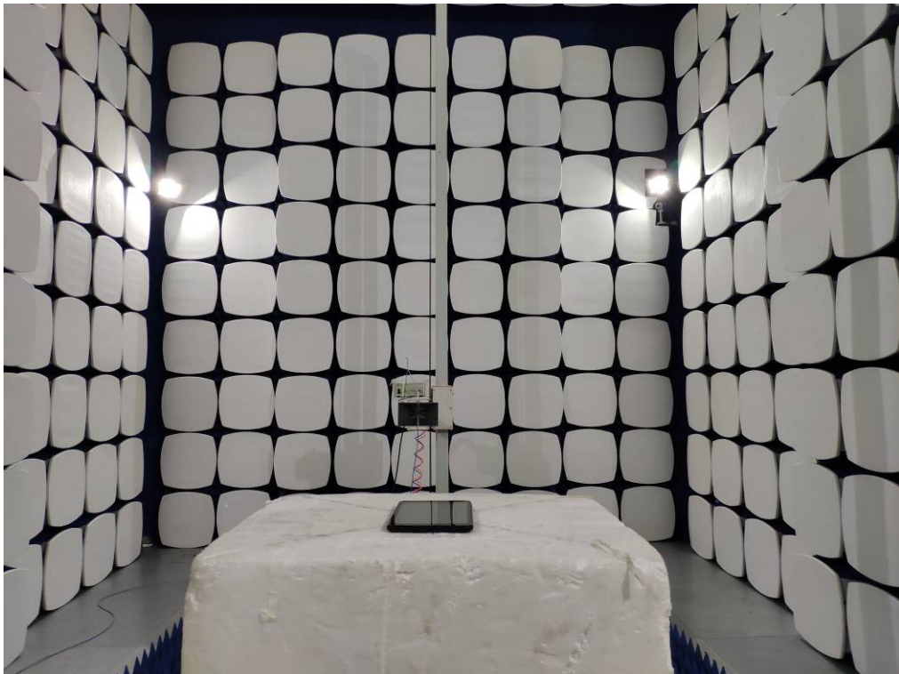
Radiated emission Setup photo (Above 1G)
