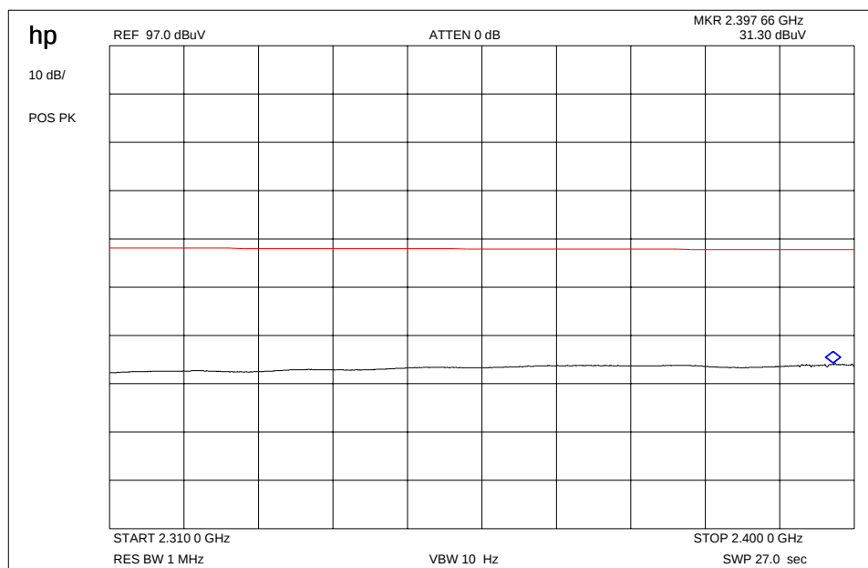
Plot 3: Restricted Band 2310 MHz – 2390 MHz
