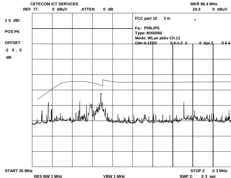
Plot 15: 0.03 – 0.2 GHz horizontal (highest channel)
