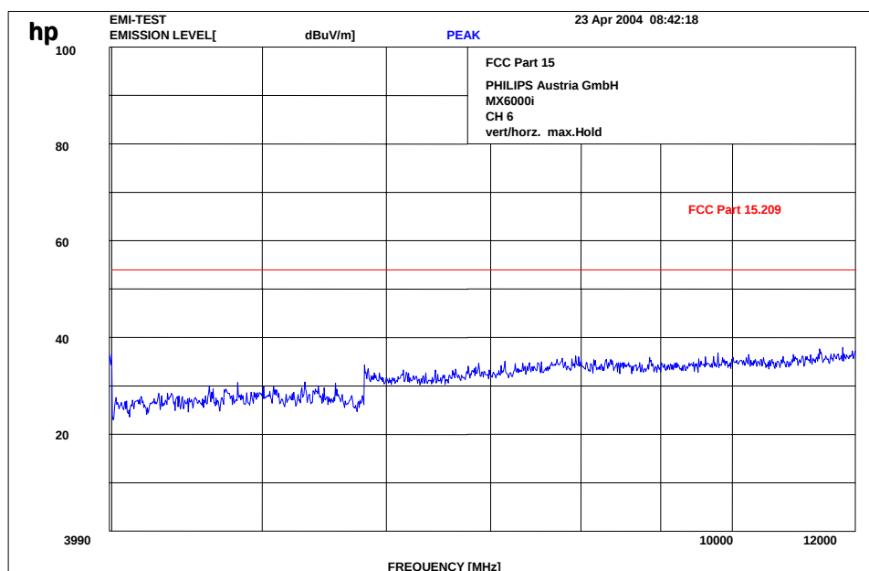
Plot 13: 4- 12 GHz vertical / horizontal (middle channel)
