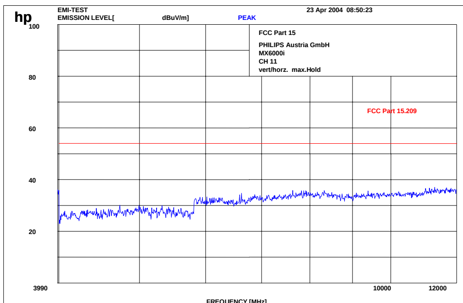
Plot 19: 4- 12 GHz vertical / horizontal (highest channel)
