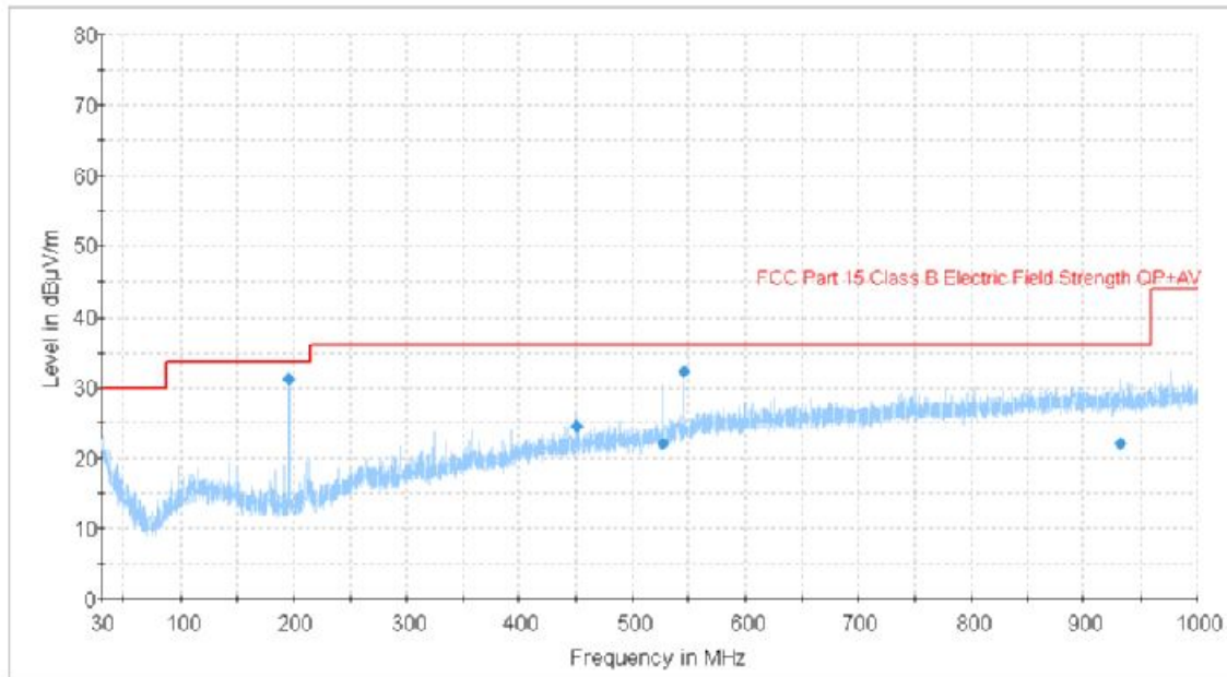
Plot 8: 30 MHz – 1000 MHz horizontal / vertical (highest channel)
