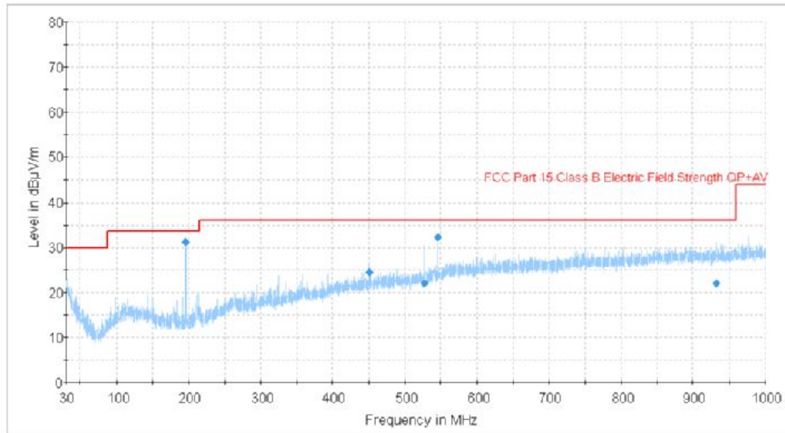
Plot 5: 30 - 1000 MHz vertical / horizontal (middle channel)
