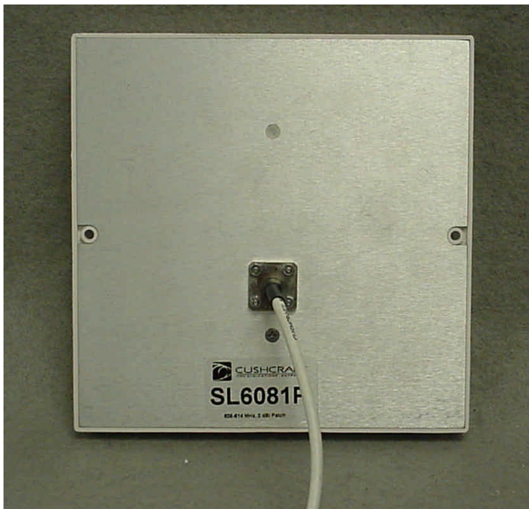
Photo 12. Patch Antenna, Bottom View
