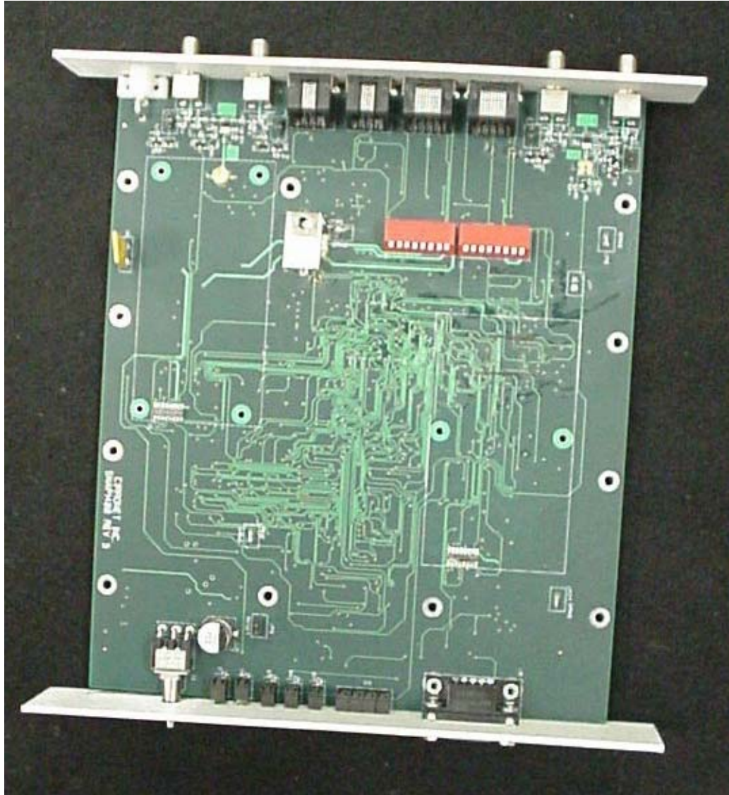
Photo 4. EUT, Top View, Cover Opened, Transceiver Removed
