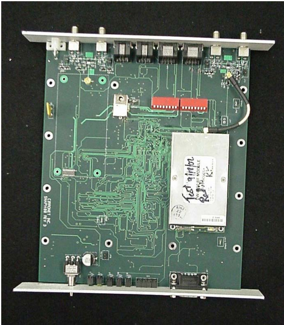
Photo 3. EUT, Top View, Cover Opened
