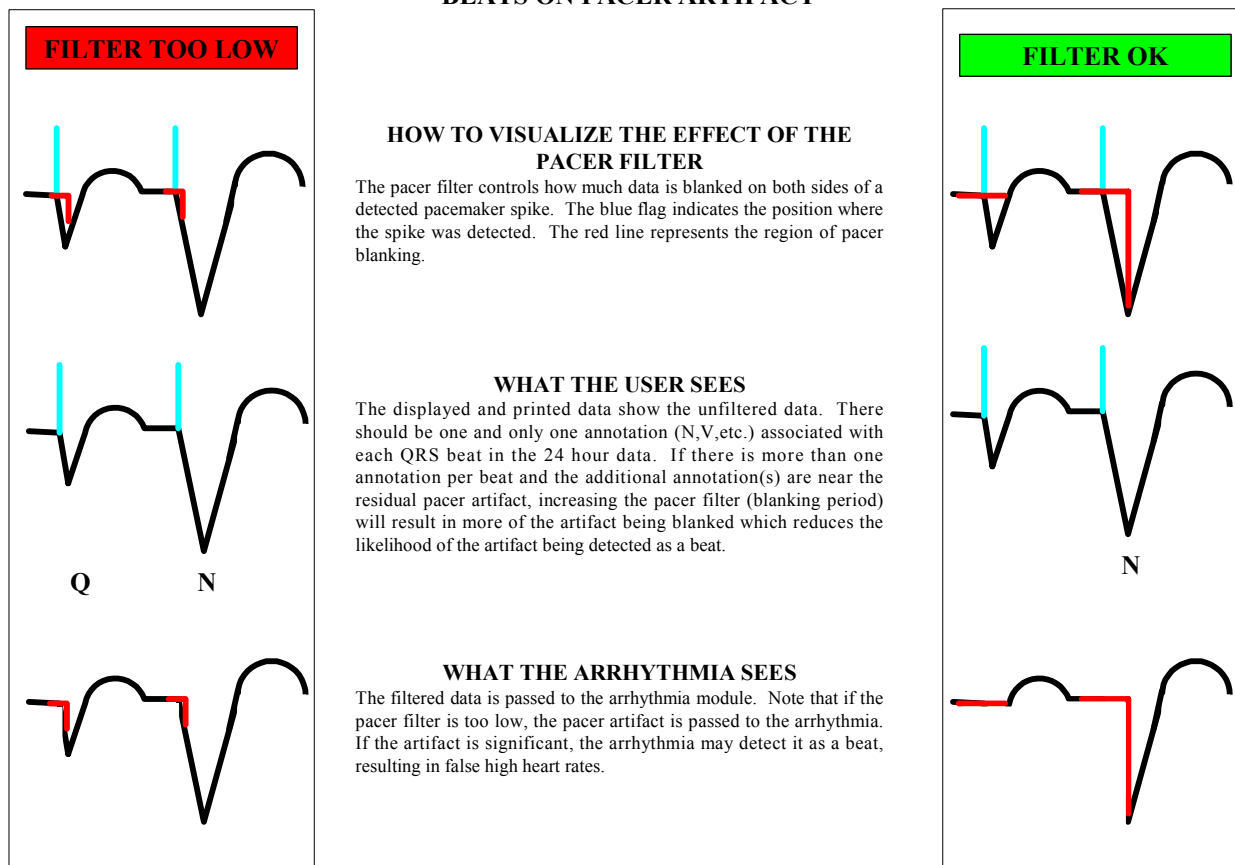
Fig. 43. False High Rates Due to Detection of Beats on Pacer Artifact
