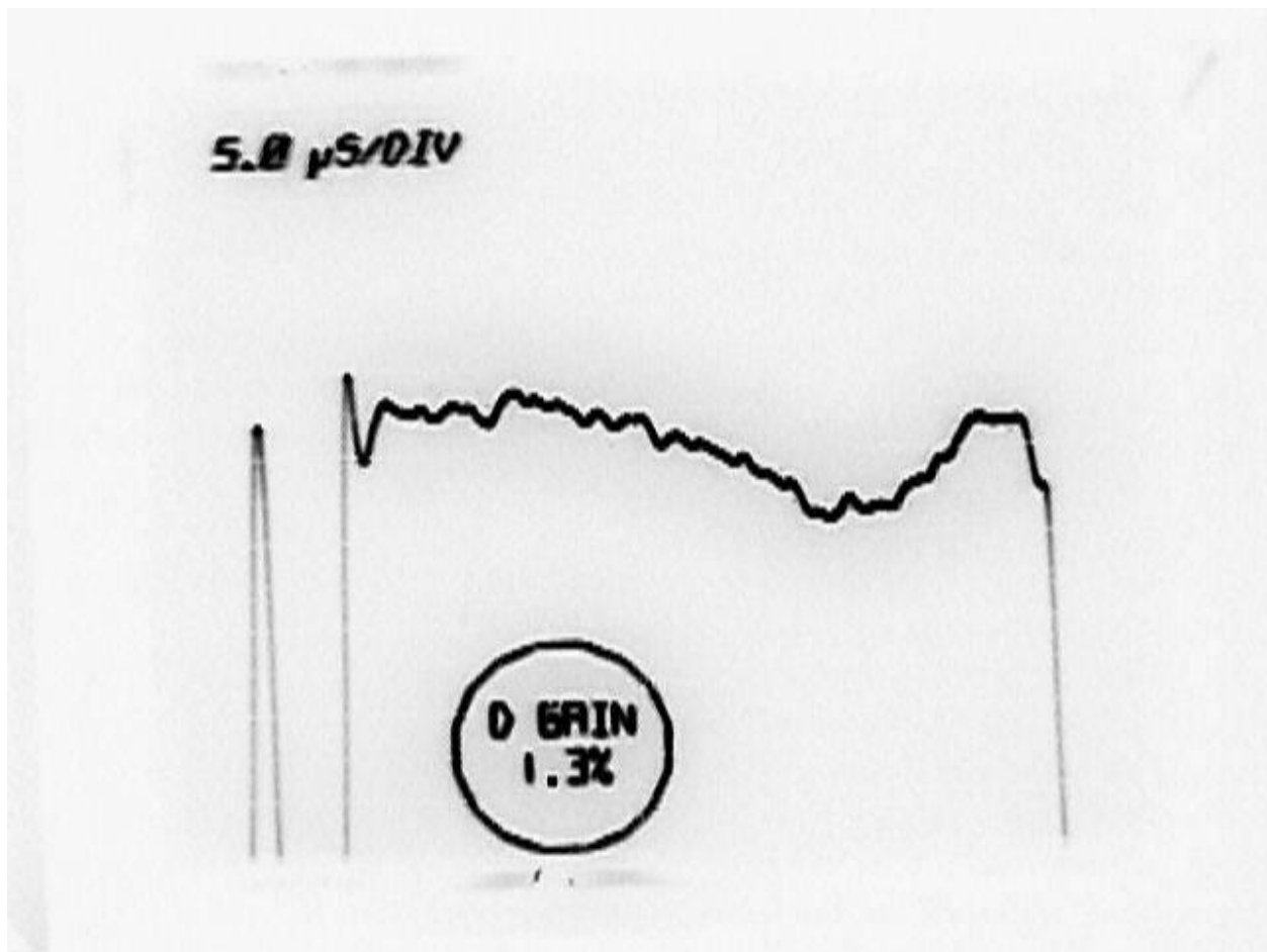
Differential Gain
