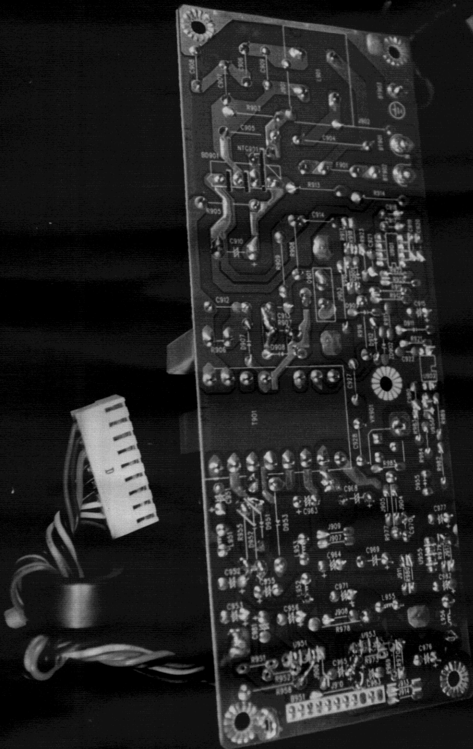
FCC ID. : BR8DV-821 E.U.T. : DIGITAL SATELLITE RECEIVER Solder View of Power PCB
