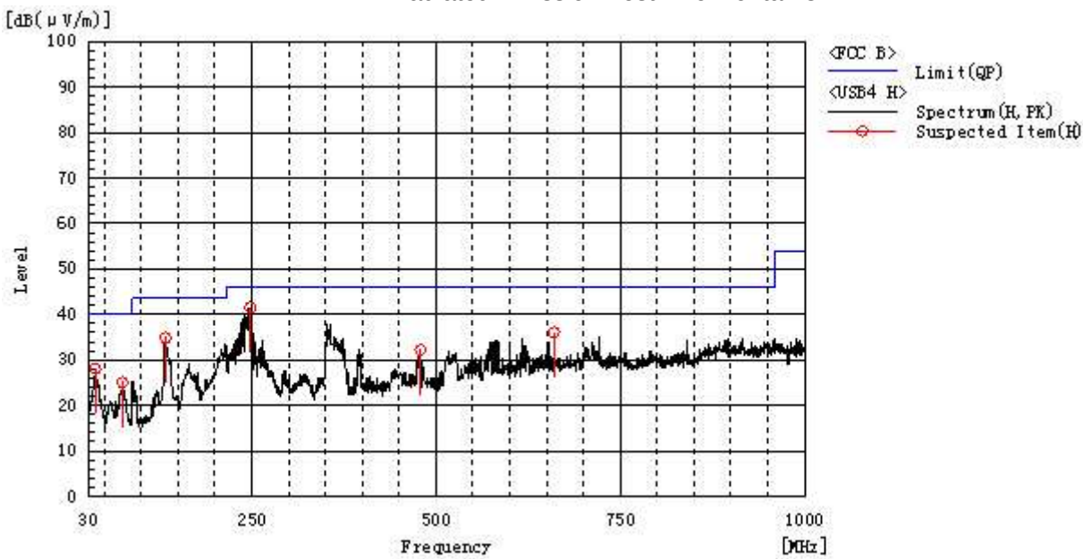
Radiated Emission Test –Horizontal -3m
