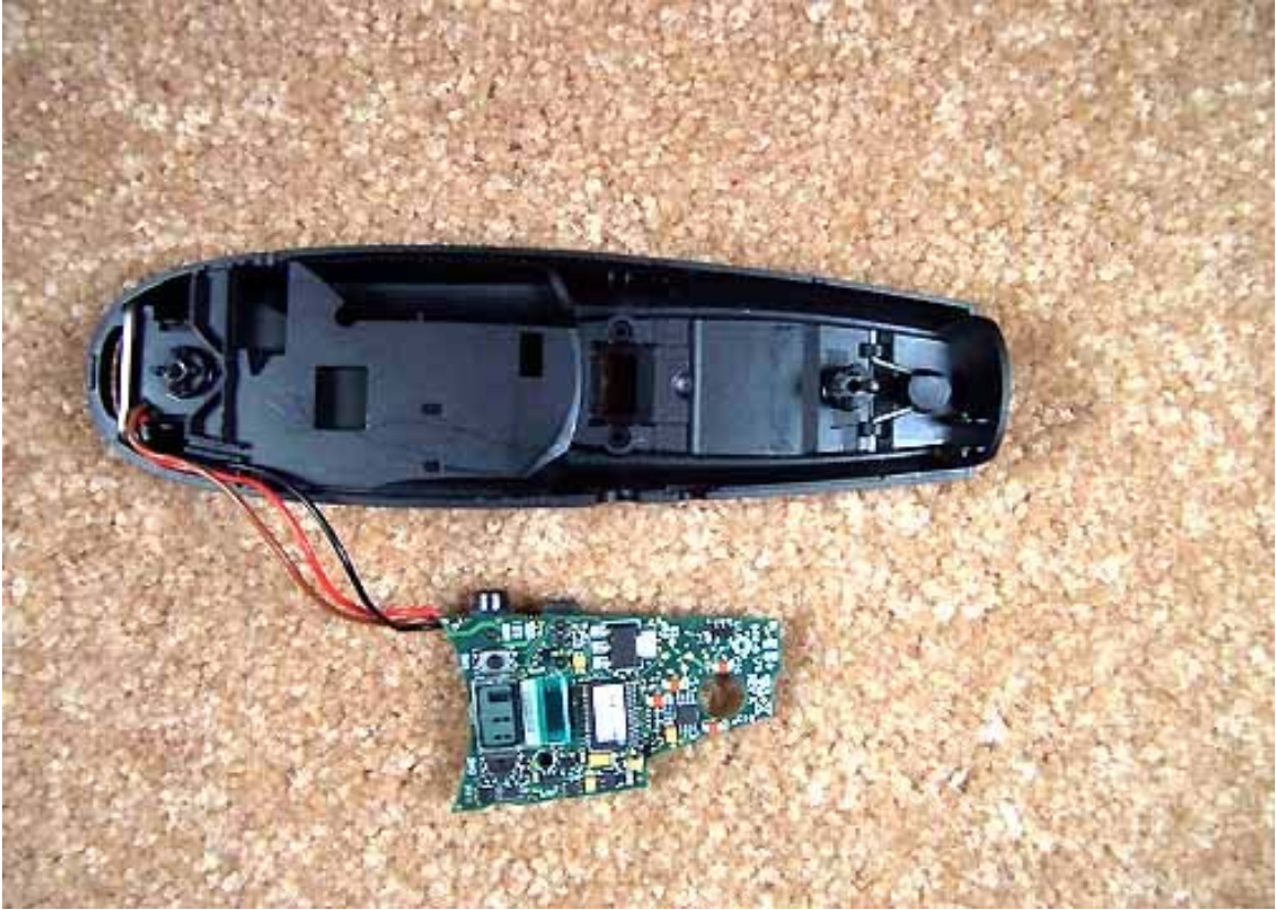
Small PCB Bottom
