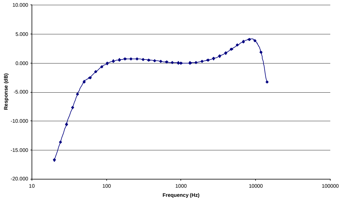
Audio Frequency Response Phonic Ear PE921T Channel 45
