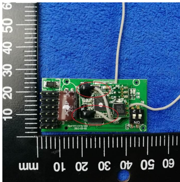
Antenna View
