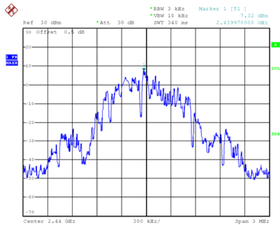
GFSK(ANT 1): channel 12
