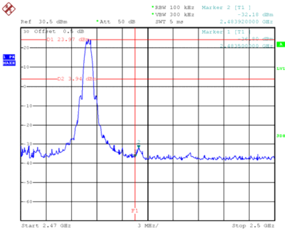
GFSK(ANT 2): Band edge-right side
