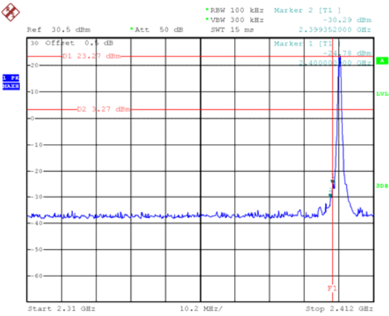
GFSK(ANT 2): Band edge-left side
