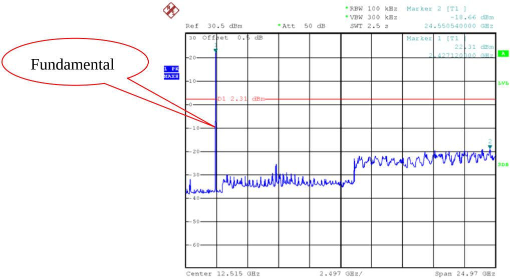
Middle Channel
