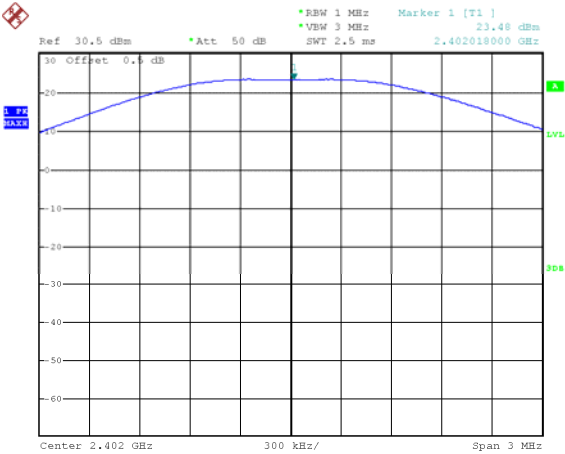
GFSK(ANT 1): channel 0
