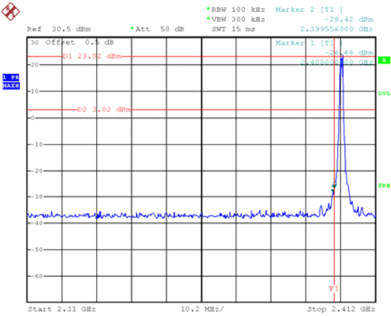
GFSK(ANT 1): Band edge-left side
