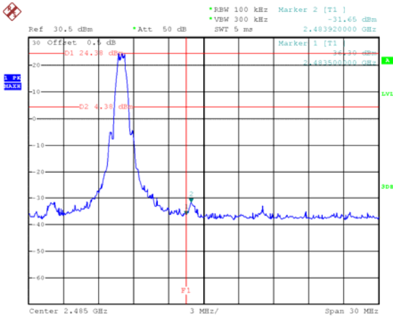
GFSK(ANT 1): Band edge-right side
