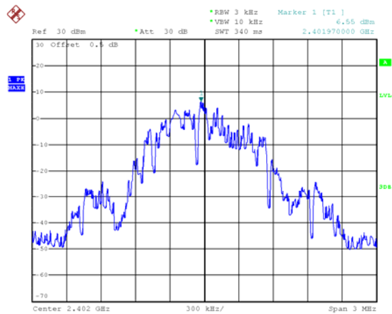
GFSK(ANT 1): channel 0
