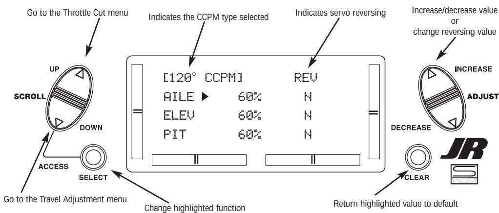
Screen showing 120° CCPM Swashplate selection
