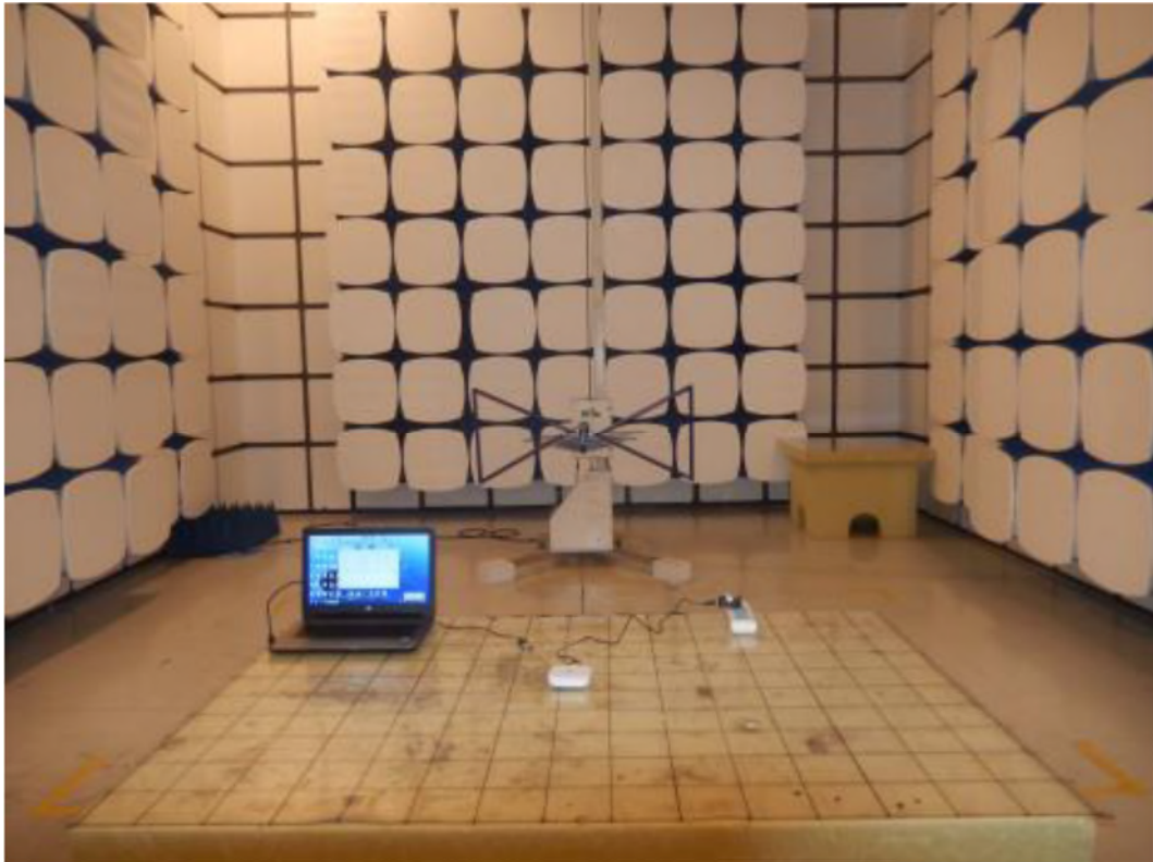
Photograph 1: Set-up for Radiated Spurious Emission, 30MHz - 1GHz
