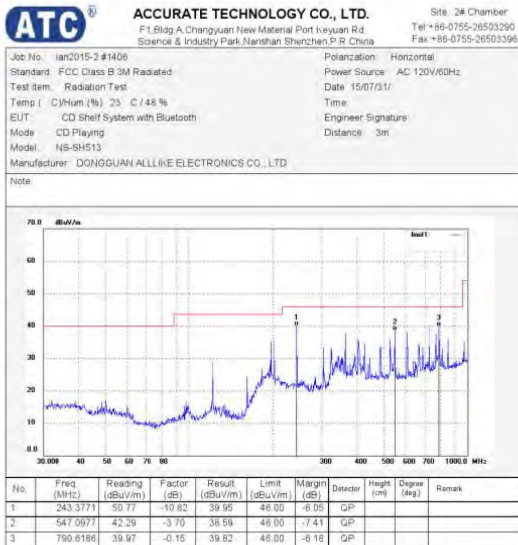
Figure 24: Test figure of Radiated Emissions
