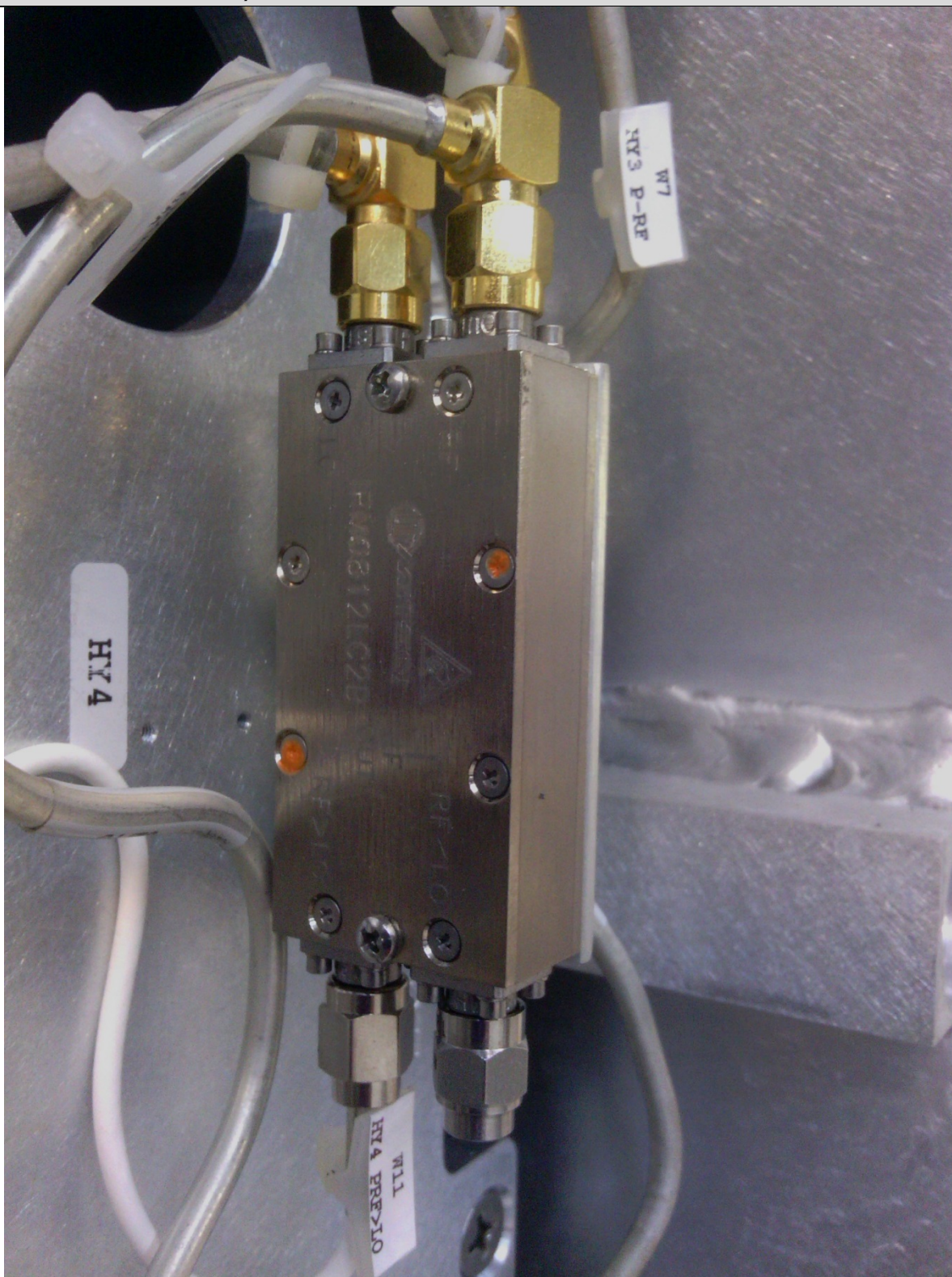
IMAGE REJECT MIXER, IRM0812LC2B-1
