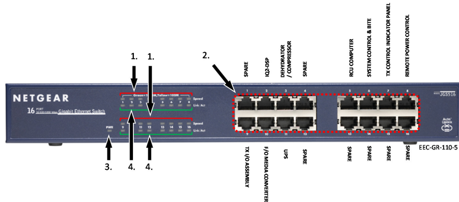
Figure 9. 16-Port Gigabit Ethernet Switch (JGS816)
