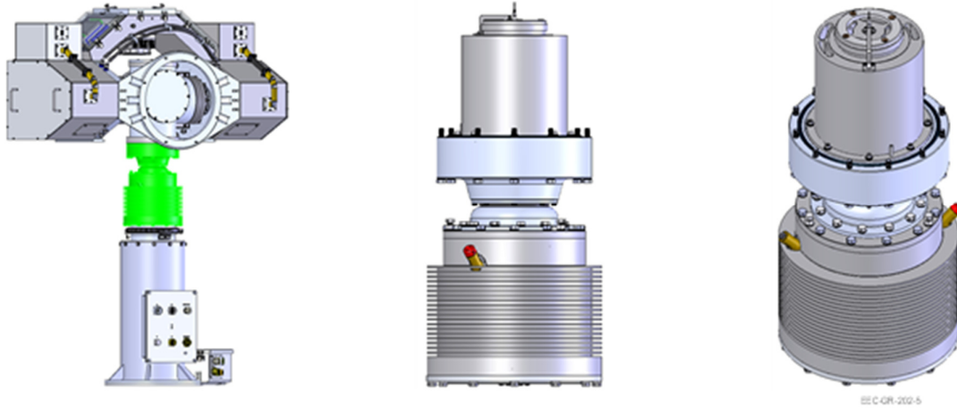
Figure 20. Azimuth Assembly (135887-100)
