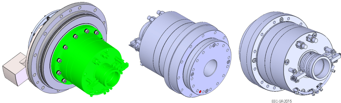
Figure 25. Actuator Unit (135782-100)
