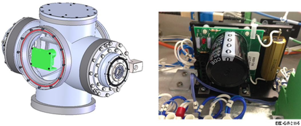
Figure 29. Regeneration Clamp (1000-327)
