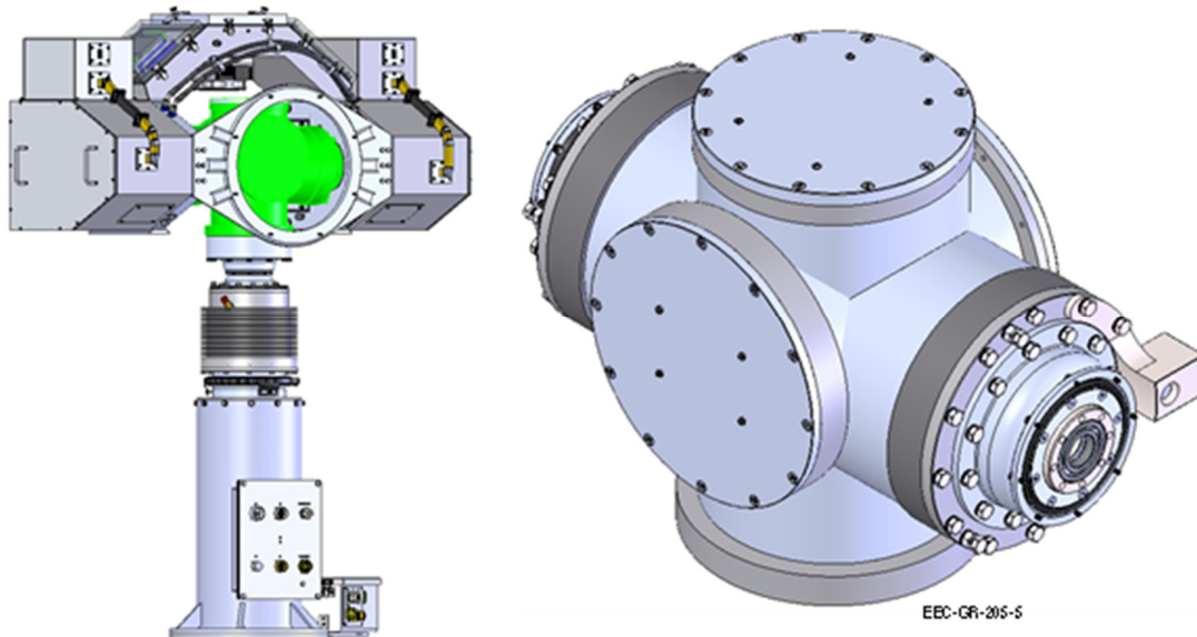
Figure 23. Elevation Assembly (135952-100)
