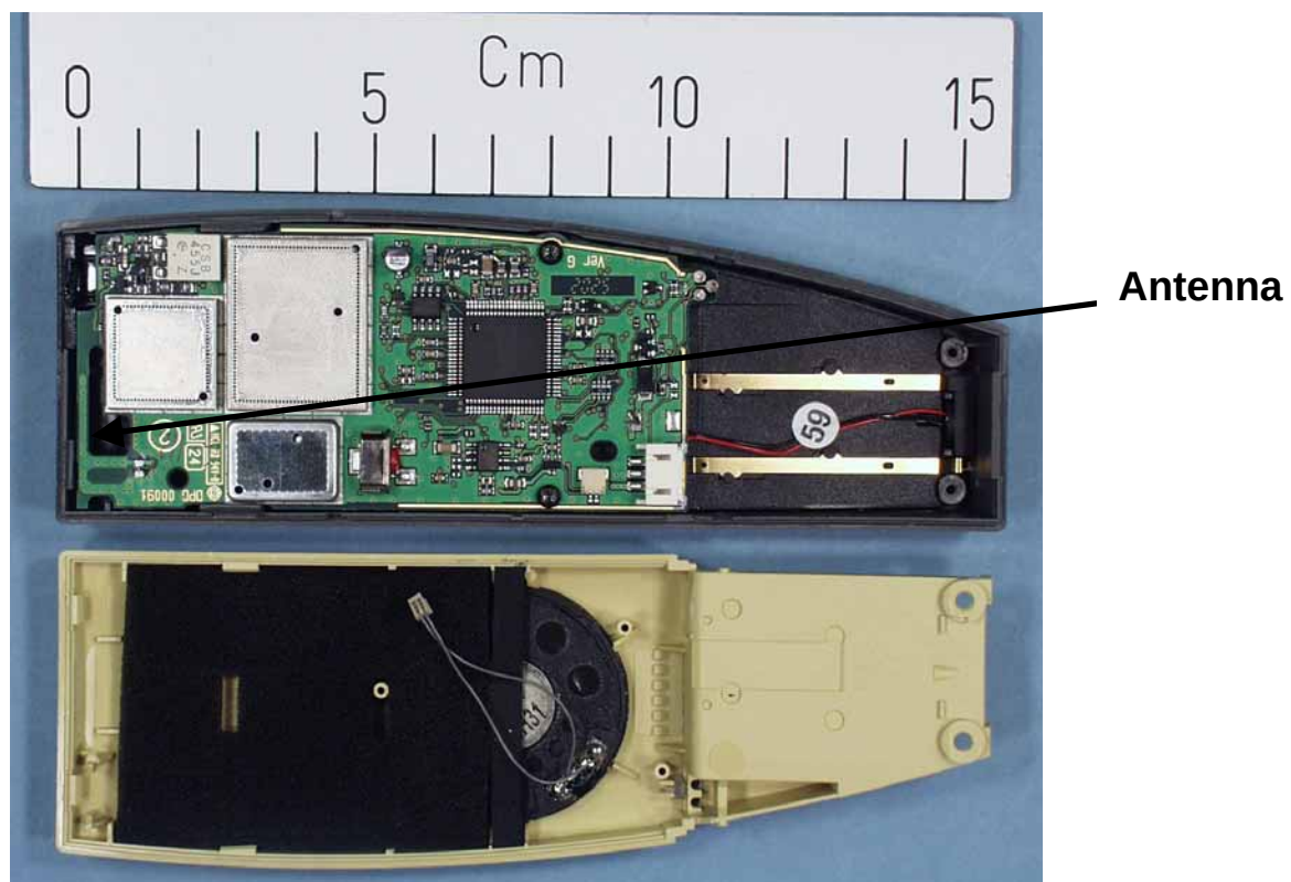
Handset, print layout
