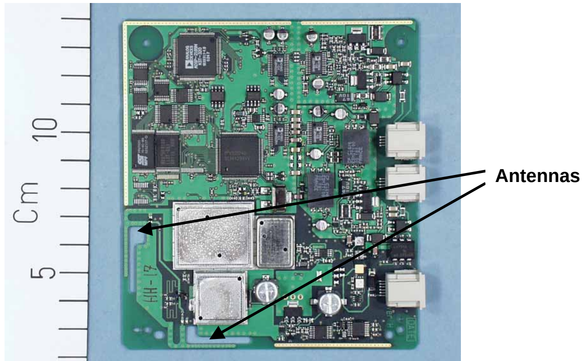
Base, print layout
