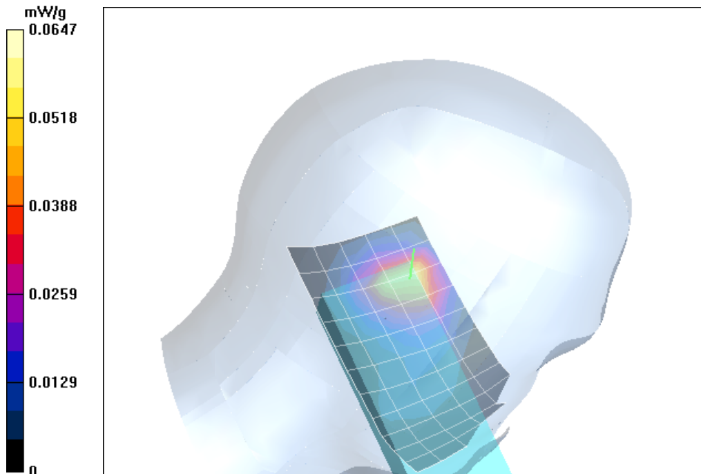
Fig. 2: SAR distribution for 2450 MHz, channel 041, tilted position, left side of head. (02.07.2003; Ambient Temperature: 21.1° C; Liquid Temperature : 19.2° C).
