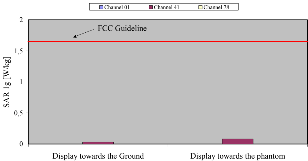
Fig. 9: The measured head phantom SAR values for the Bang & Olufsen BeoCom 1 for 2.4 GHz in comparison to the FCC exposure limit.
