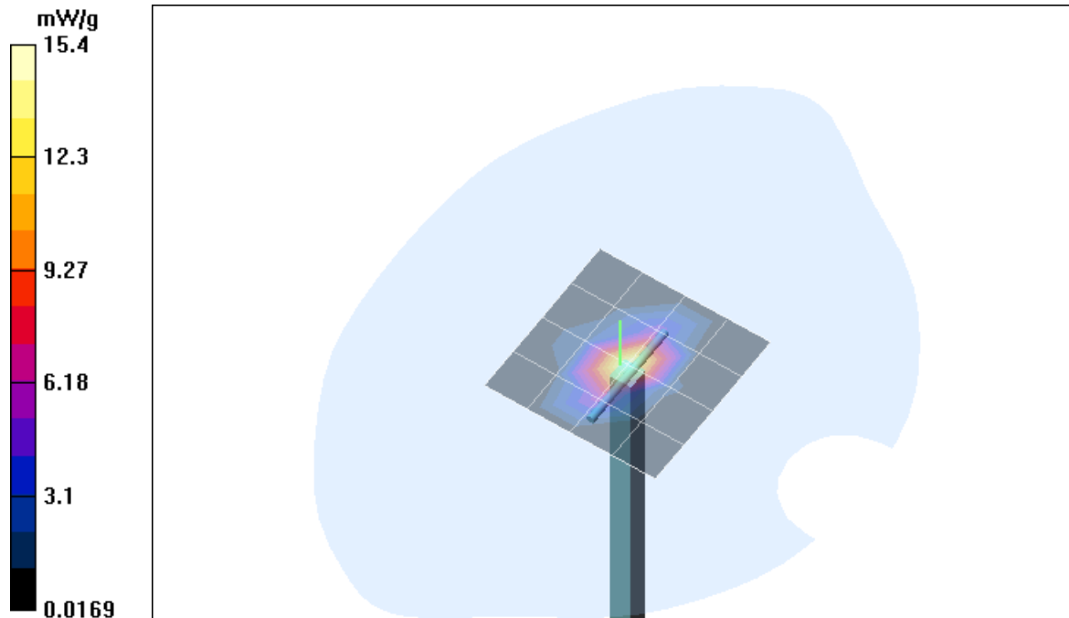
Fig. 11: Validation measurement 2450 MHz Head (July 02, 2003), coarse grid. Ambient Temperature: 21.1° C, Liquid Temperature: 20.5° C.
