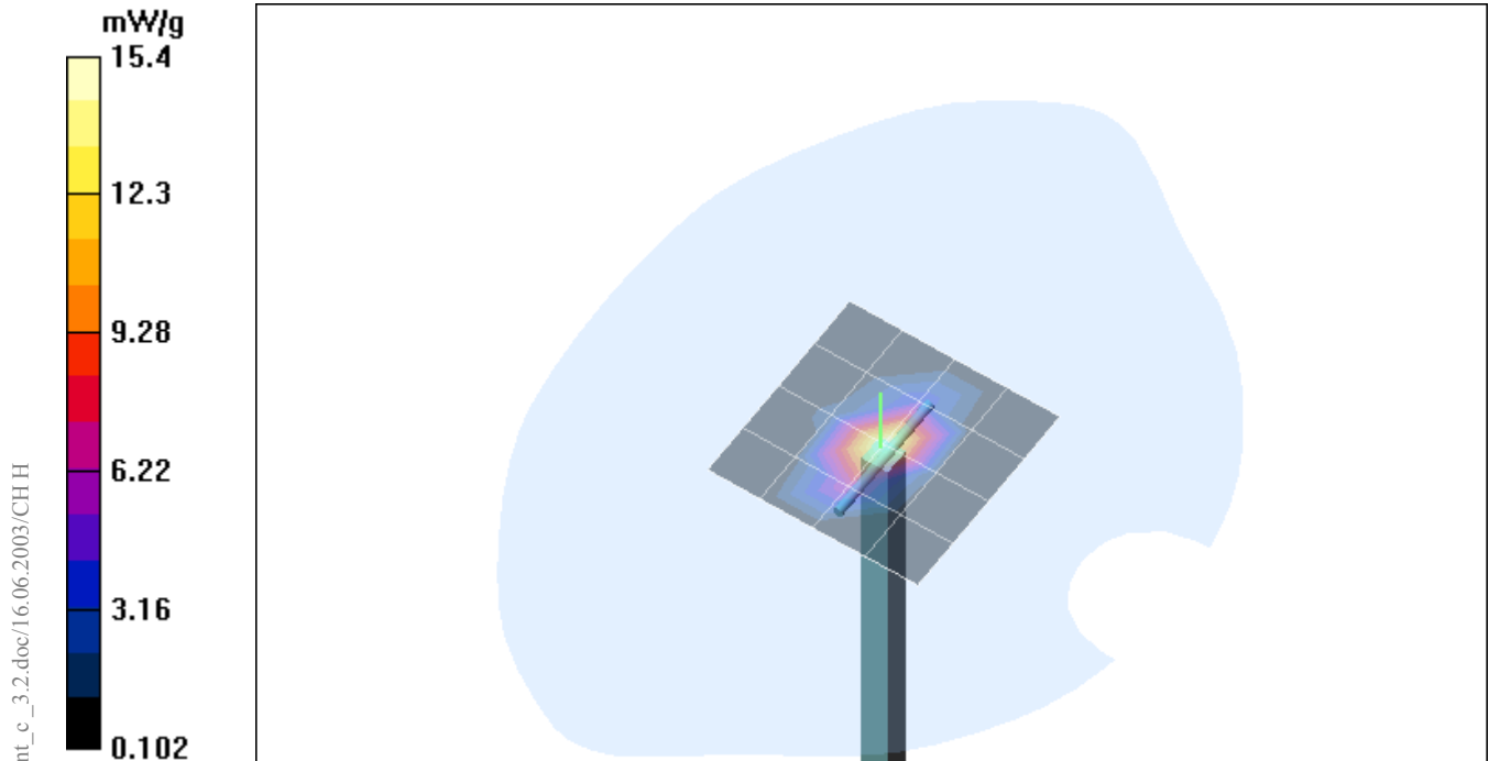
Fig. 12: Validation measurement 2450 MHz body (July 03, 2003), coarse grid. Ambient Temperature: 21.0° C, Liquid Temperature: 20.6° C.
